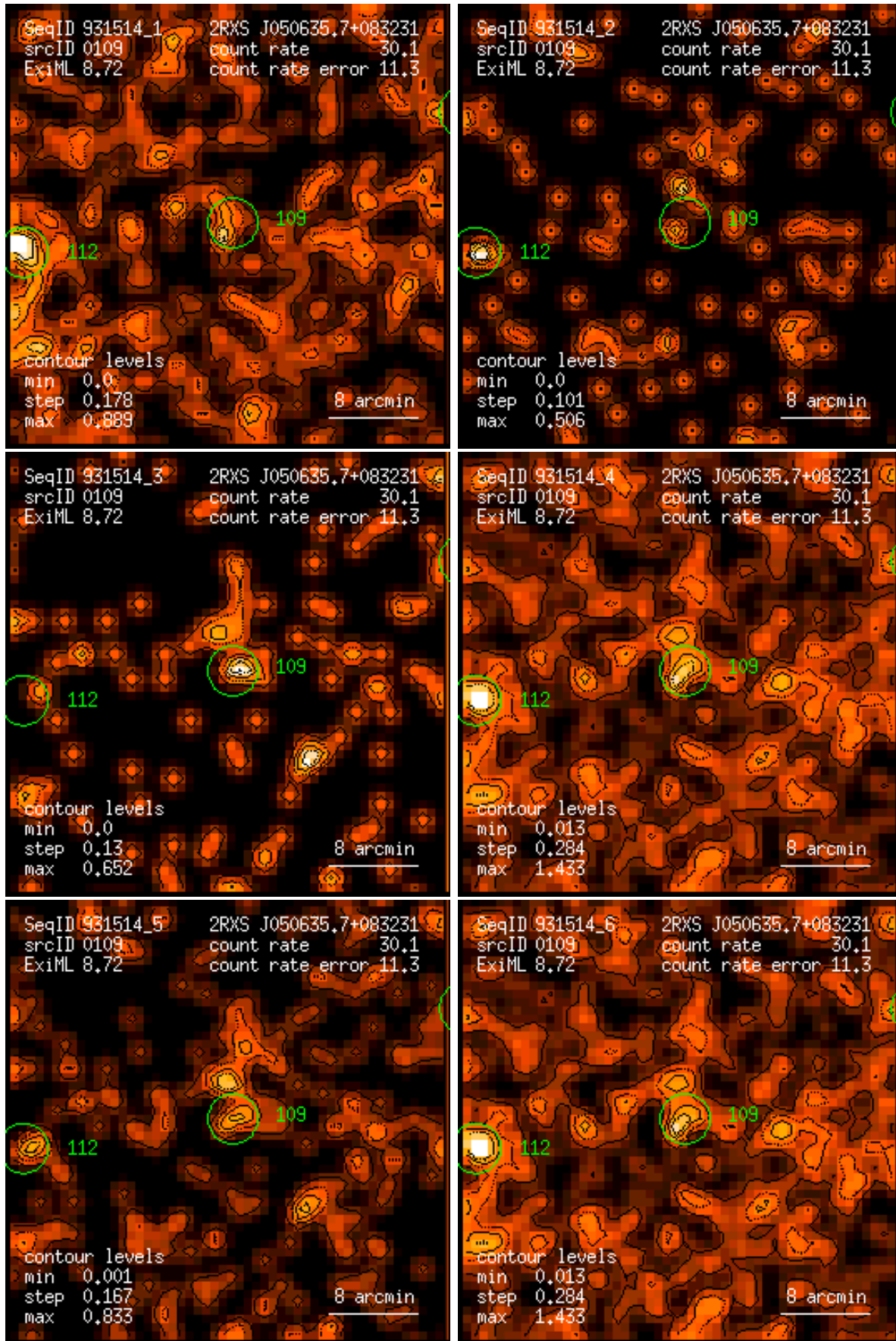
Figure 109: RASS 931514: detection 0109: band rate images, Gaussian filter: (1) PSPC channels 11 – 41, (2) 52 – 90, (3) 91 – 201, (4) 11 – 235, (5) 52 – 201, (6) 11 – 201. Broad band rates in counts/ks. Band rate contour levels in counts/ks/arcmin 2 .
