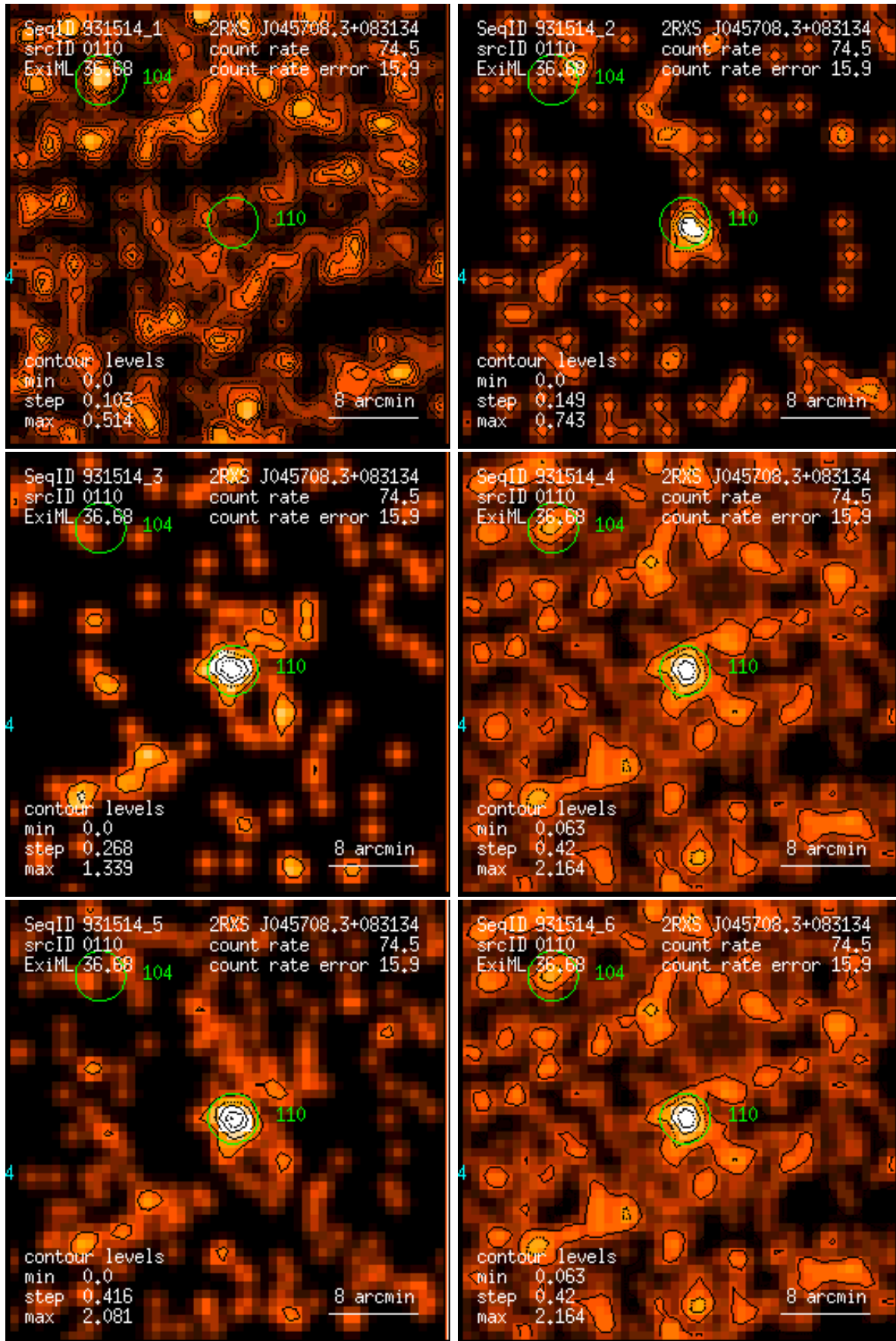
Figure 110: RASS 931514: detection 0110: band rate images, Gaussian filter: (1) PSPC channels 11 – 41, (2) 52 – 90, (3) 91 – 201, (4) 11 – 235, (5) 52 – 201, (6) 11 – 201. Broad band rates in counts/ks. Band rate contour levels in counts/ks/arcmin 2 .
