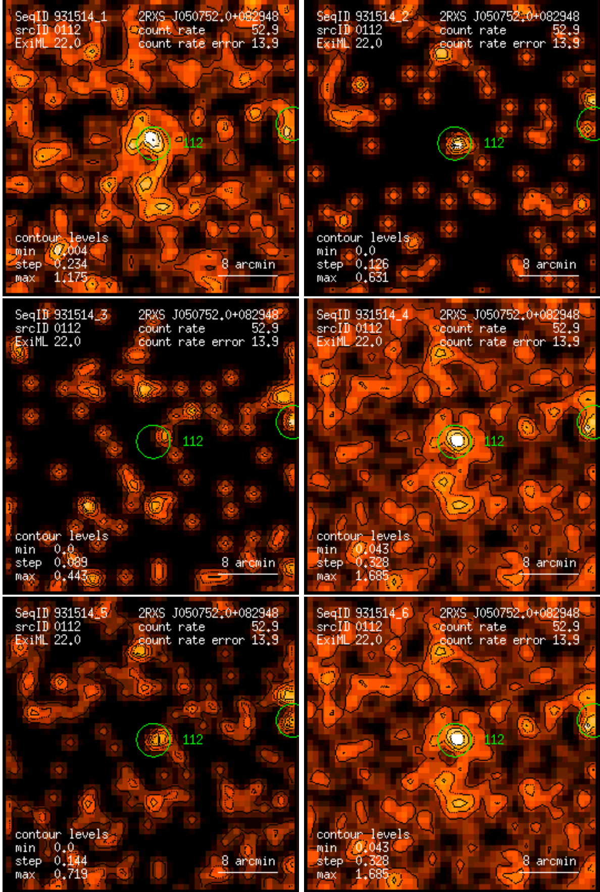
Figure 112: RASS 931514: detection 0112: band rate images, Gaussian filter: (1) PSPC channels 11 – 41, (2) 52 – 90, (3) 91 – 201, (4) 11 – 235, (5) 52 – 201, (6) 11 – 201. Broad band rates in counts/ks. Band rate contour levels in counts/ks/arcmin 2 .
