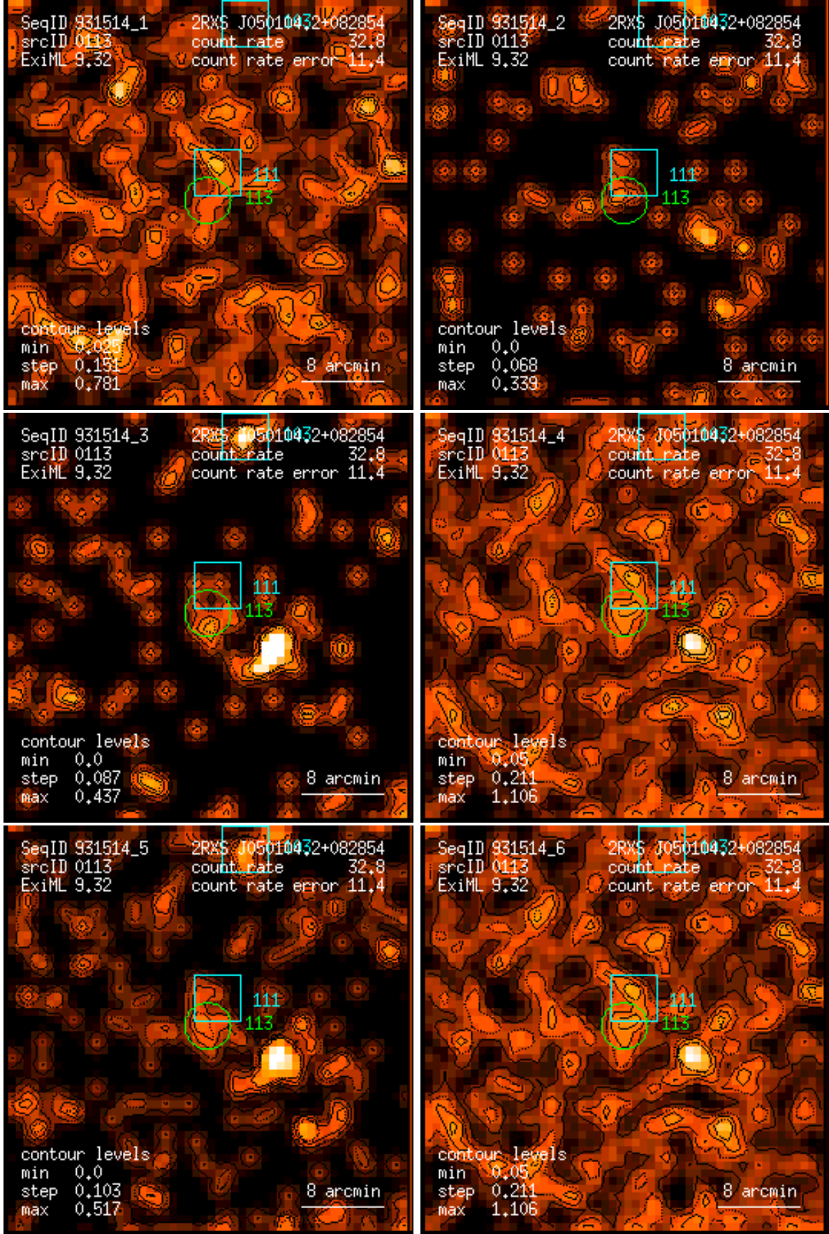
Figure 113: RASS 931514: detection 0113: band rate images, Gaussian filter: (1) PSPC channels 11 – 41, (2) 52 – 90, (3) 91 – 201, (4) 11 – 235, (5) 52 – 201, (6) 11 – 201. Broad band rates in counts/ks. Band rate contour levels in counts/ks/arcmin 2 .
