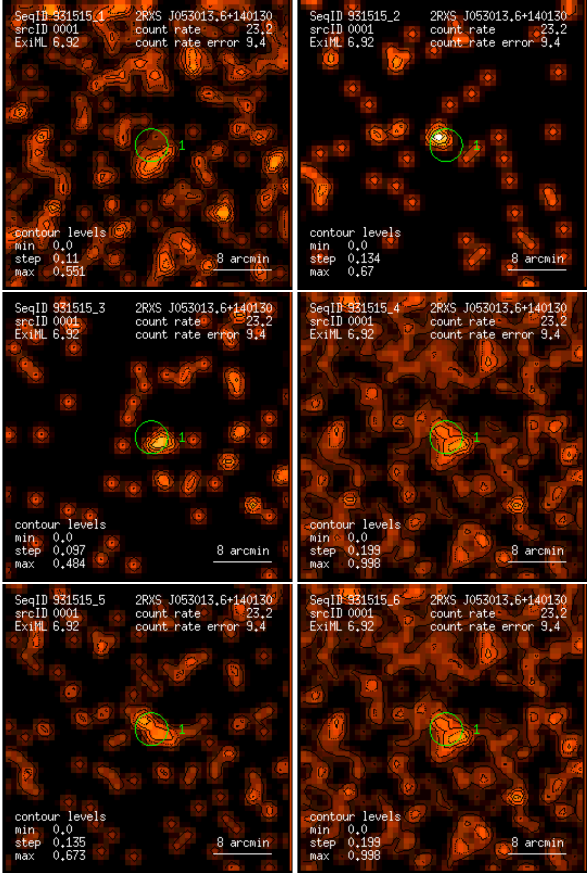
Figure 1: RASS 931515: detection 0001: band rate images, Gaussian filter: (1) PSPC channels 11 – 41, (2) 52 – 90, (3) 91 – 201, (4) 11 – 235, (5) 52 – 201, (6) 11 – 201. Broad band rates in counts/ks. Band rate contour levels in counts/ks/arcmin 2 .
