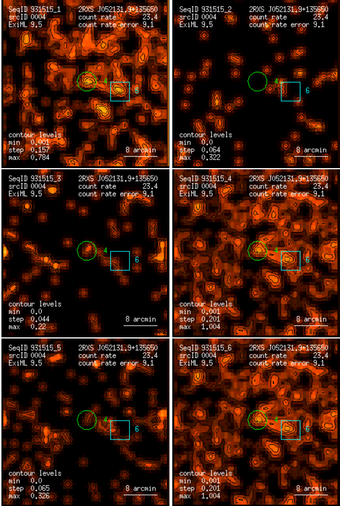
Figure 4: RASS 931515: detection 0004: band rate images, Gaussian filter: (1) PSPC channels 11 – 41, (2) 52 – 90, (3) 91 – 201, (4) 11 – 235, (5) 52 – 201, (6) 11 – 201. Broad band rates in counts/ks. Band rate contour levels in counts/ks/arcmin 2 .
