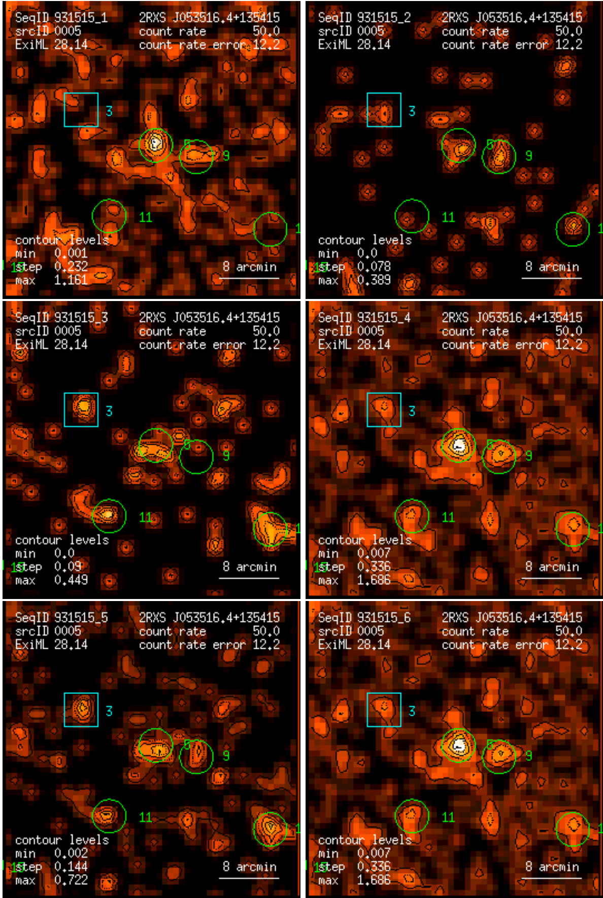
Figure 5: RASS 931515: detection 0005: band rate images, Gaussian filter: (1) PSPC channels 11 – 41, (2) 52 – 90, (3) 91 – 201, (4) 11 – 235, (5) 52 – 201, (6) 11 – 201. Broad band rates in counts/ks. Band rate contour levels in counts/ks/arcmin 2 .
