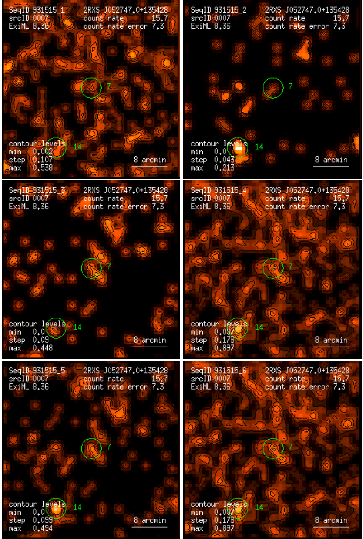
Figure 7: RASS 931515: detection 0007: band rate images, Gaussian filter: (1) PSPC channels 11 – 41, (2) 52 – 90, (3) 91 – 201, (4) 11 – 235, (5) 52 – 201, (6) 11 – 201. Broad band rates in counts/ks. Band rate contour levels in counts/ks/arcmin 2 .
