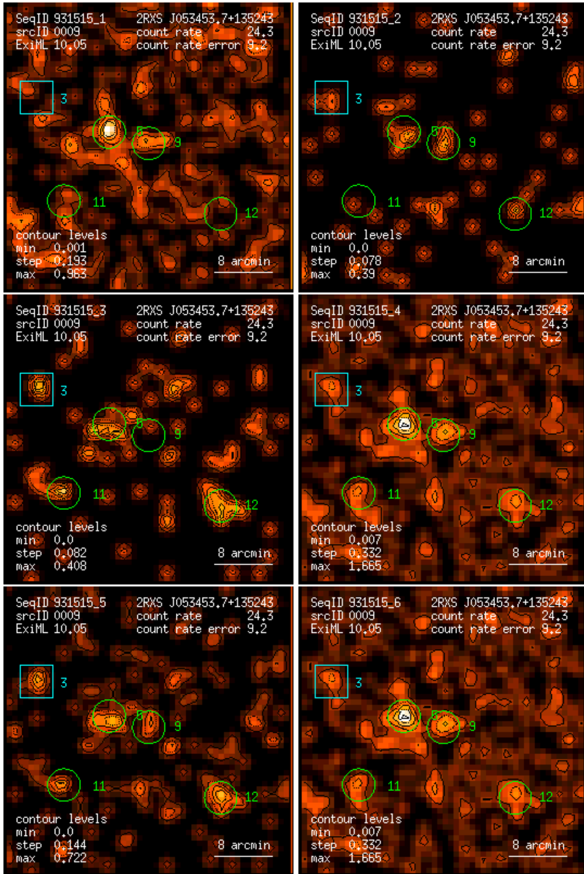
Figure 9: RASS 931515: detection 0009: band rate images, Gaussian filter: (1) PSPC channels 11 – 41, (2) 52 – 90, (3) 91 – 201, (4) 11 – 235, (5) 52 – 201, (6) 11 – 201. Broad band rates in counts/ks. Band rate contour levels in counts/ks/arcmin 2 .
