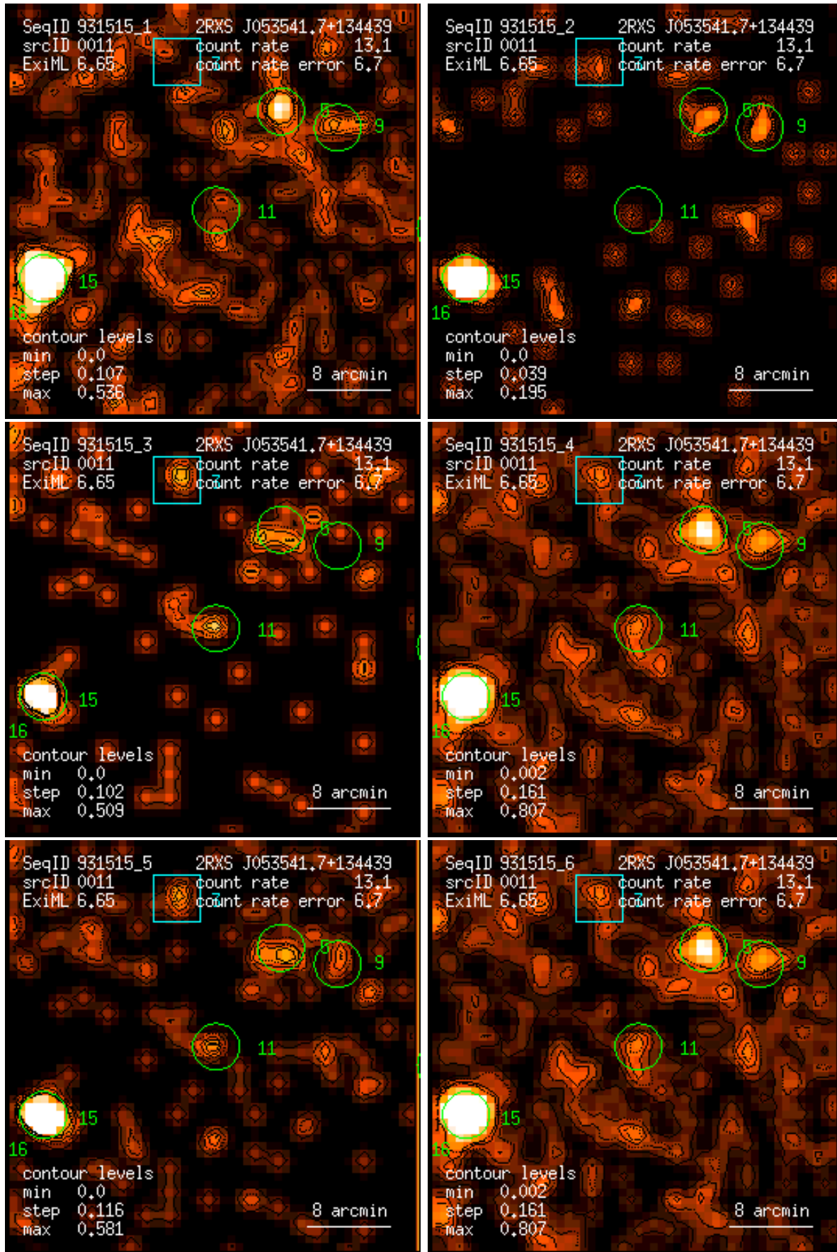
Figure 11: RASS 931515: detection 0011: band rate images, Gaussian filter: (1) PSPC channels 11 – 41, (2) 52 – 90, (3) 91 – 201, (4) 11 – 235, (5) 52 – 201, (6) 11 – 201. Broad band rates in counts/ks. Band rate contour levels in counts/ks/arcmin 2 .
