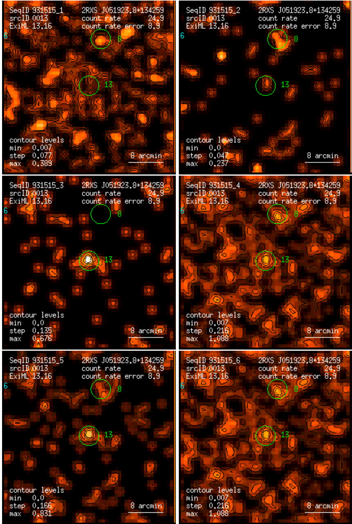
Figure 13: RASS 931515: detection 0013: band rate images, Gaussian filter: (1) PSPC channels 11 – 41, (2) 52 – 90, (3) 91 – 201, (4) 11 – 235, (5) 52 – 201, (6) 11 – 201. Broad band rates in counts/ks. Band rate contour levels in counts/ks/arcmin 2 .
