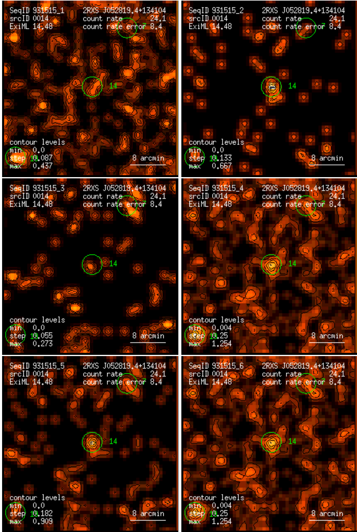
Figure 14: RASS 931515: detection 0014: band rate images, Gaussian filter: (1) PSPC channels 11 – 41, (2) 52 – 90, (3) 91 – 201, (4) 11 – 235, (5) 52 – 201, (6) 11 – 201. Broad band rates in counts/ks. Band rate contour levels in counts/ks/arcmin 2 .
