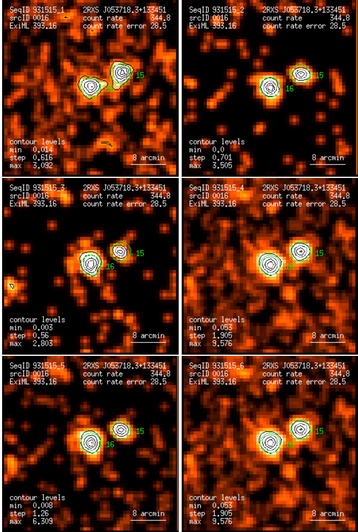
Figure 16: RASS 931515: detection 0016: band rate images, Gaussian filter: (1) PSPC channels 11 – 41, (2) 52 – 90, (3) 91 – 201, (4) 11 – 235, (5) 52 – 201, (6) 11 – 201. Broad band rates in counts/ks. Band rate contour levels in counts/ks/arcmin 2 .
