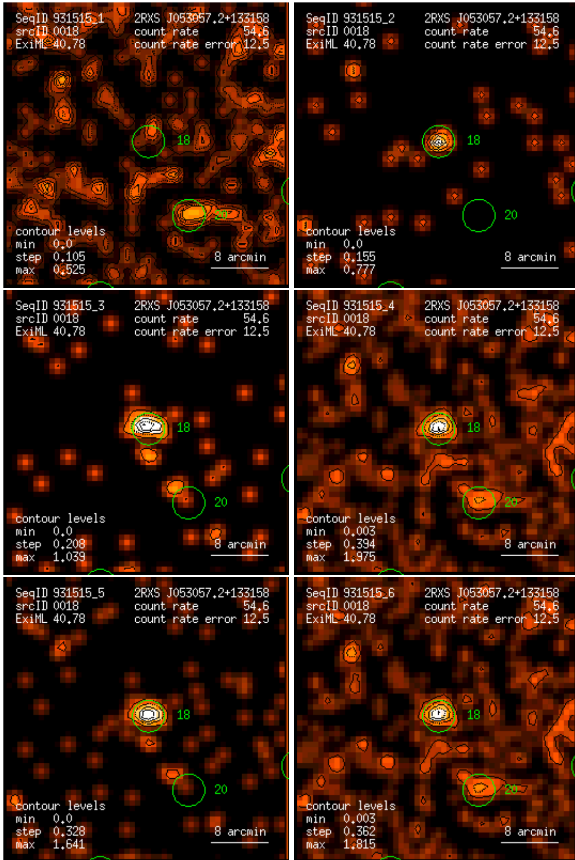
Figure 18: RASS 931515: detection 0018: band rate images, Gaussian filter: (1) PSPC channels 11 – 41, (2) 52 – 90, (3) 91 – 201, (4) 11 – 235, (5) 52 – 201, (6) 11 – 201. Broad band rates in counts/ks. Band rate contour levels in counts/ks/arcmin 2 .
