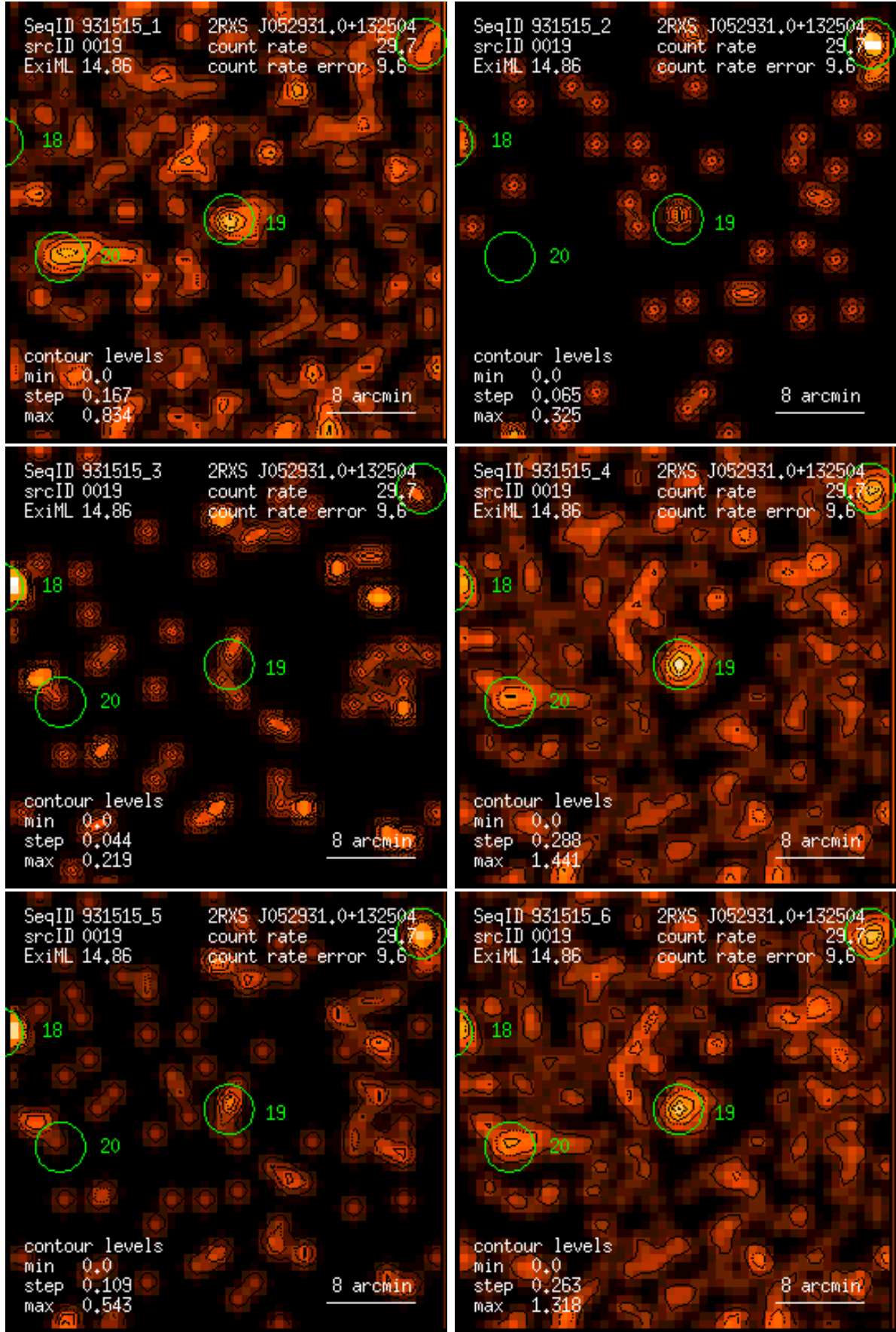
Figure 19: RASS 931515: detection 0019: band rate images, Gaussian filter: (1) PSPC channels 11 – 41, (2) 52 – 90, (3) 91 – 201, (4) 11 – 235, (5) 52 – 201, (6) 11 – 201. Broad band rates in counts/ks. Band rate contour levels in counts/ks/arcmin 2 .
