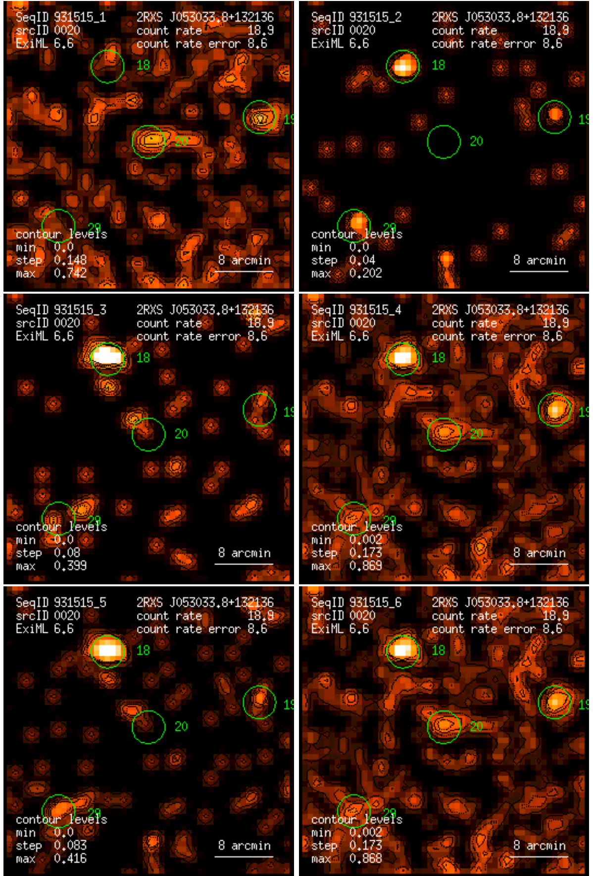
Figure 20: RASS 931515: detection 0020: band rate images, Gaussian filter: (1) PSPC channels 11 – 41, (2) 52 – 90, (3) 91 – 201, (4) 11 – 235, (5) 52 – 201, (6) 11 – 201. Broad band rates in counts/ks. Band rate contour levels in counts/ks/arcmin 2 .
