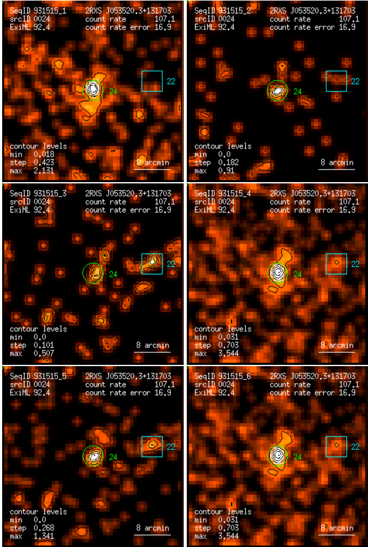
Figure 24: RASS 931515: detection 0024: band rate images, Gaussian filter: (1) PSPC channels 11 – 41, (2) 52 – 90, (3) 91 – 201, (4) 11 – 235, (5) 52 – 201, (6) 11 – 201. Broad band rates in counts/ks. Band rate contour levels in counts/ks/arcmin 2 .
