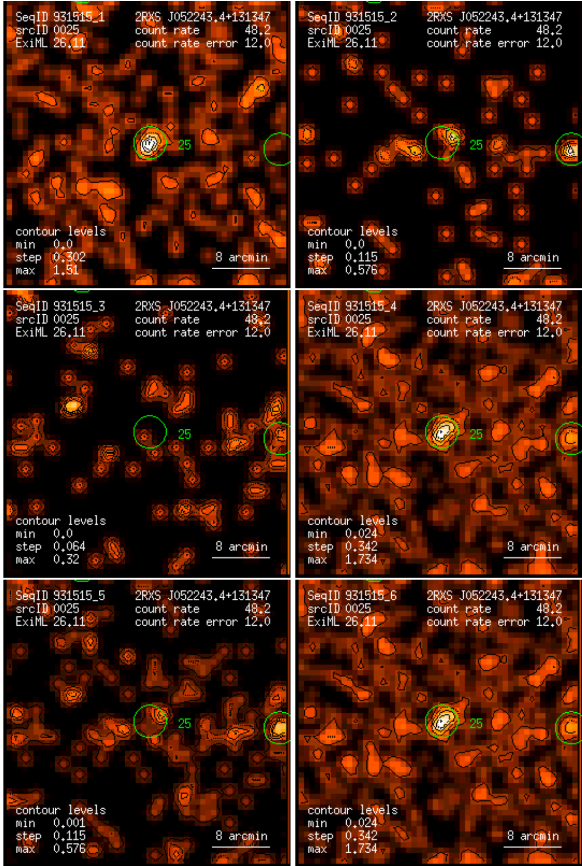
Figure 25: RASS 931515: detection 0025: band rate images, Gaussian filter: (1) PSPC channels 11 – 41, (2) 52 – 90, (3) 91 – 201, (4) 11 – 235, (5) 52 – 201, (6) 11 – 201. Broad band rates in counts/ks. Band rate contour levels in counts/ks/arcmin 2 .
