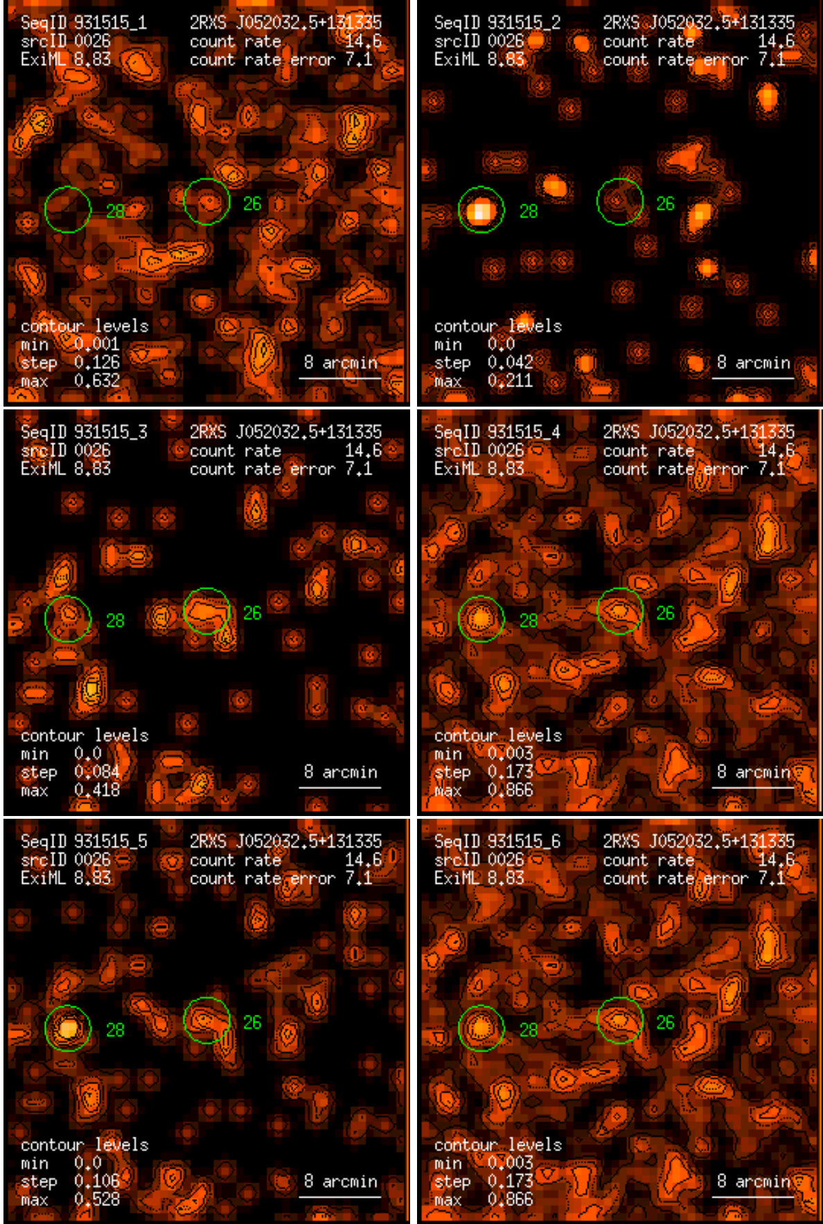
Figure 26: RASS 931515: detection 0026: band rate images, Gaussian filter: (1) PSPC channels 11 – 41, (2) 52 – 90, (3) 91 – 201, (4) 11 – 235, (5) 52 – 201, (6) 11 – 201. Broad band rates in counts/ks. Band rate contour levels in counts/ks/arcmin 2 .
