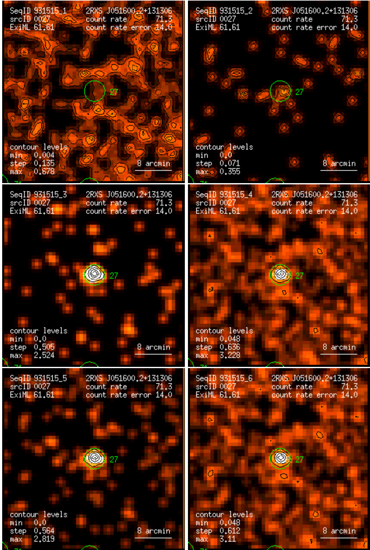
Figure 27: RASS 931515: detection 0027: band rate images, Gaussian filter: (1) PSPC channels 11 – 41, (2) 52 – 90, (3) 91 – 201, (4) 11 – 235, (5) 52 – 201, (6) 11 – 201. Broad band rates in counts/ks. Band rate contour levels in counts/ks/arcmin 2 .
