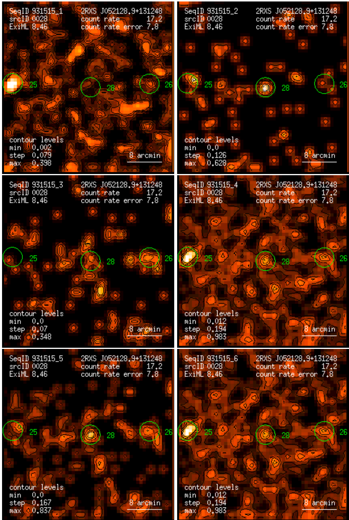
Figure 28: RASS 931515: detection 0028: band rate images, Gaussian filter: (1) PSPC channels 11 – 41, (2) 52 – 90, (3) 91 – 201, (4) 11 – 235, (5) 52 – 201, (6) 11 – 201. Broad band rates in counts/ks. Band rate contour levels in counts/ks/arcmin 2 .
