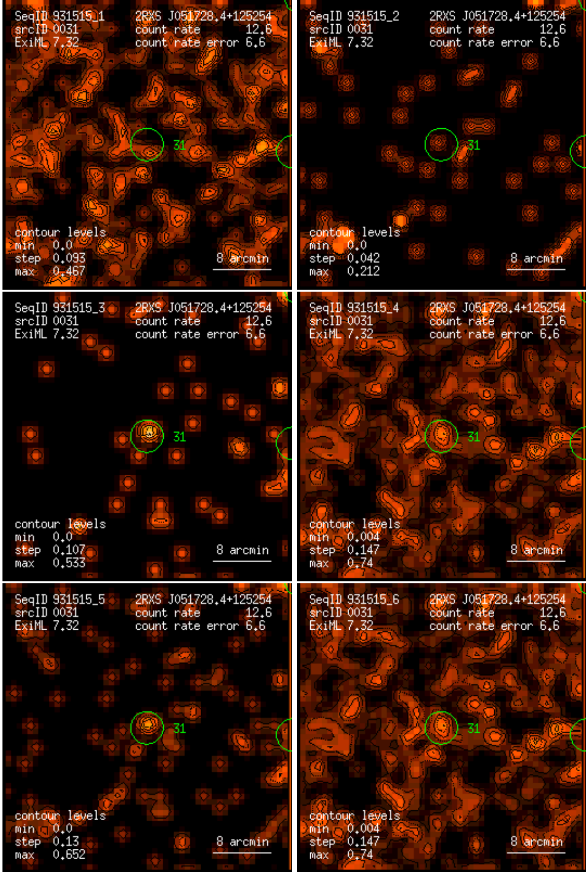
Figure 31: RASS 931515: detection 0031: band rate images, Gaussian filter: (1) PSPC channels 11 – 41, (2) 52 – 90, (3) 91 – 201, (4) 11 – 235, (5) 52 – 201, (6) 11 – 201. Broad band rates in counts/ks. Band rate contour levels in counts/ks/arcmin 2 .
