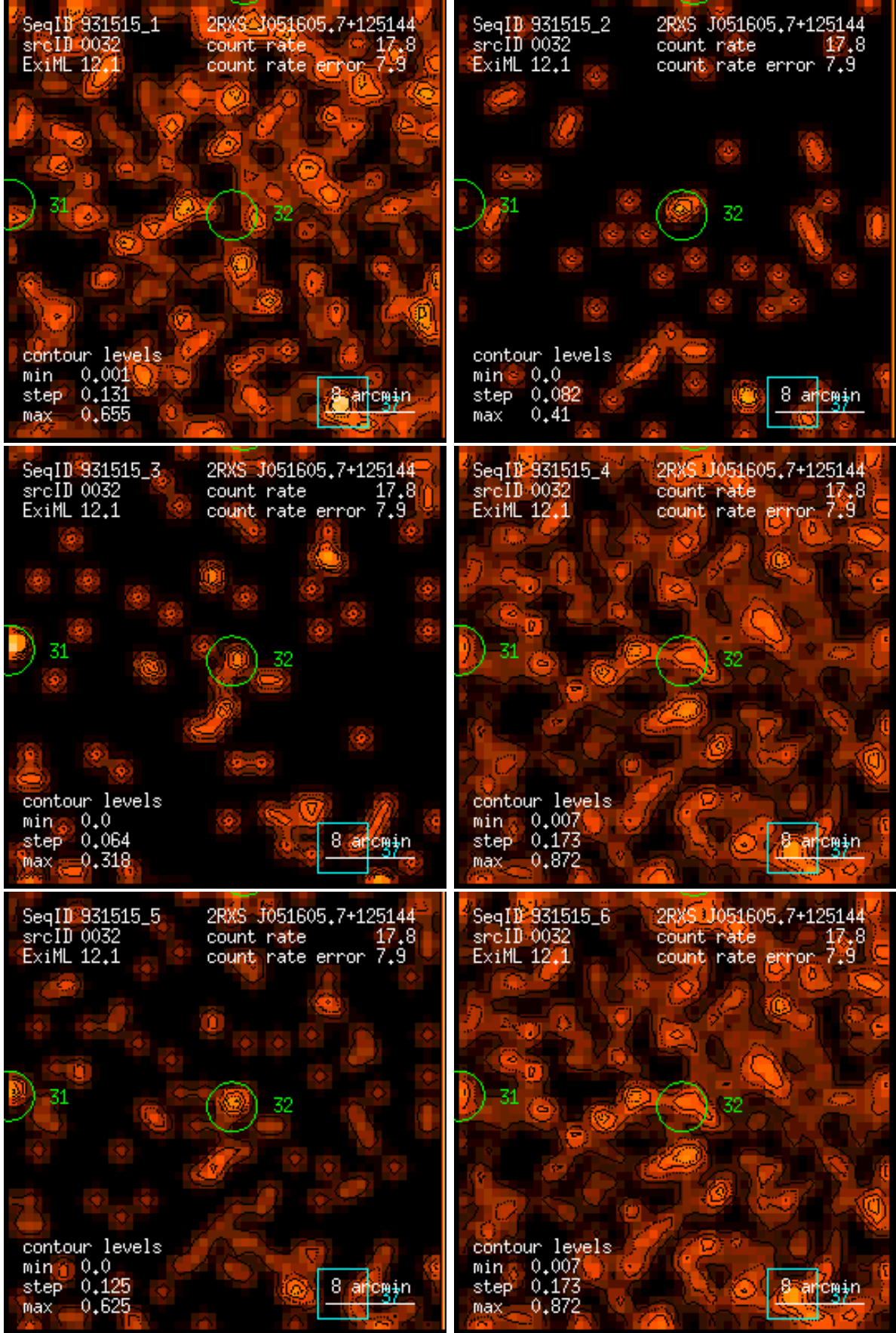
Figure 32: RASS 931515: detection 0032: band rate images, Gaussian filter: (1) PSPC channels 11 – 41, (2) 52 – 90, (3) 91 – 201, (4) 11 – 235, (5) 52 – 201, (6) 11 – 201. Broad band rates in counts/ks. Band rate contour levels in counts/ks/arcmin 2 .
