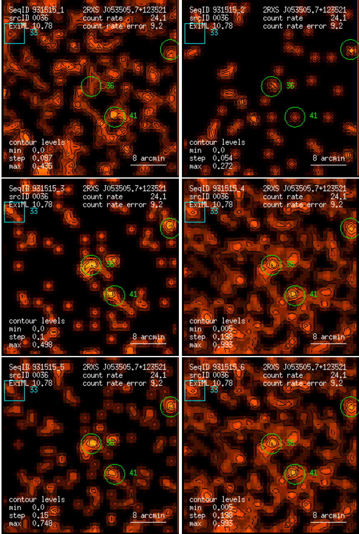
Figure 36: RASS 931515: detection 0036: band rate images, Gaussian filter: (1) PSPC channels 11 – 41, (2) 52 – 90, (3) 91 – 201, (4) 11 – 235, (5) 52 – 201, (6) 11 – 201. Broad band rates in counts/ks. Band rate contour levels in counts/ks/arcmin 2 .
