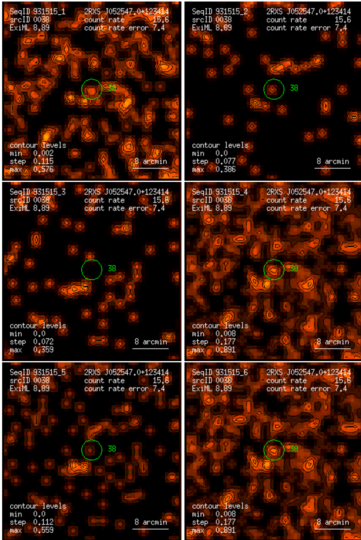
Figure 38: RASS 931515: detection 0038: band rate images, Gaussian filter: (1) PSPC channels 11 – 41, (2) 52 – 90, (3) 91 – 201, (4) 11 – 235, (5) 52 – 201, (6) 11 – 201. Broad band rates in counts/ks. Band rate contour levels in counts/ks/arcmin 2 .
