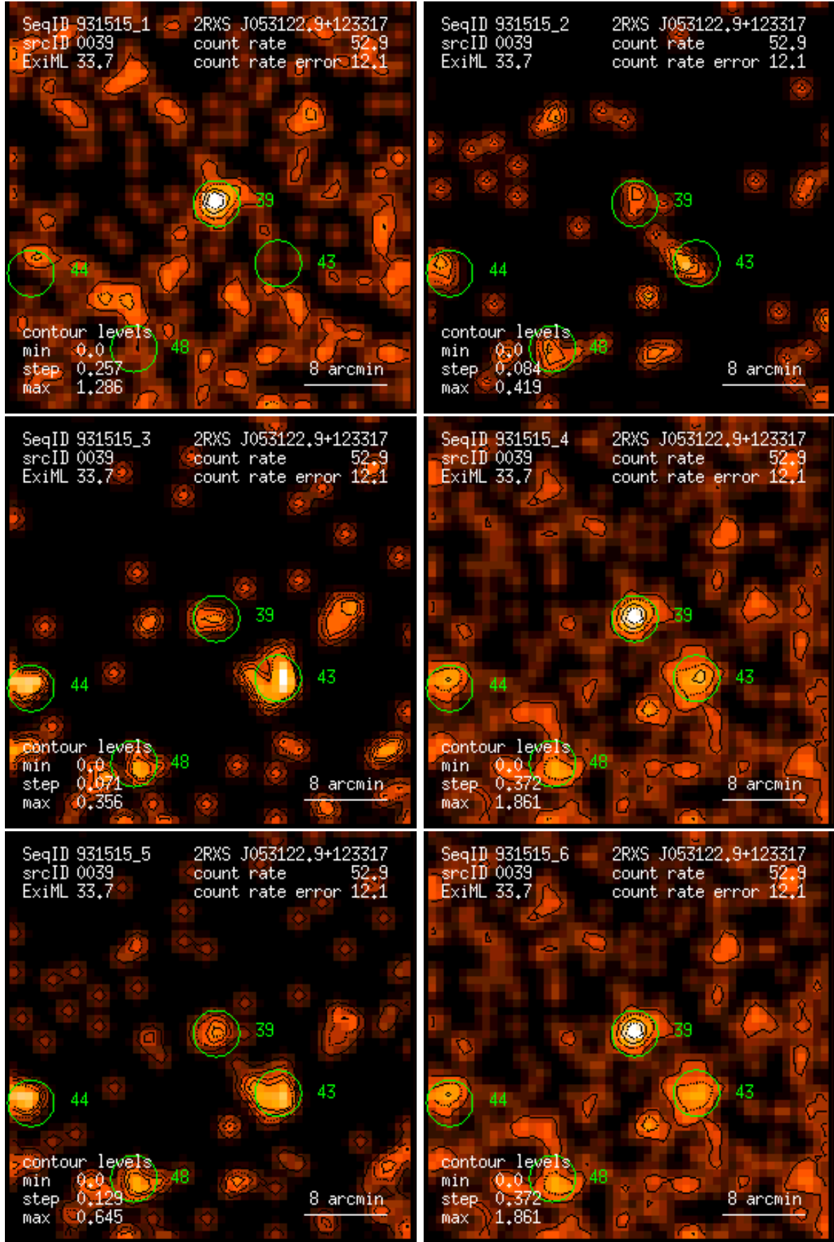
Figure 39: RASS 931515: detection 0039: band rate images, Gaussian filter: (1) PSPC channels 11 – 41, (2) 52 – 90, (3) 91 – 201, (4) 11 – 235, (5) 52 – 201, (6) 11 – 201. Broad band rates in counts/ks. Band rate contour levels in counts/ks/arcmin 2 .
