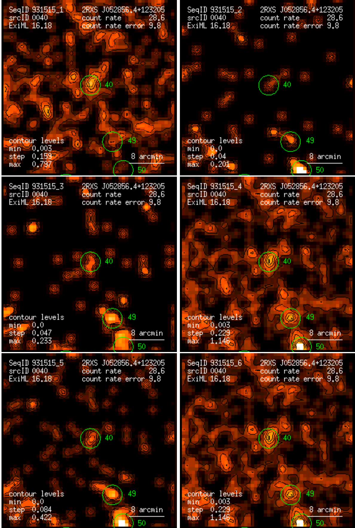
Figure 40: RASS 931515: detection 0040: band rate images, Gaussian filter: (1) PSPC channels 11 – 41, (2) 52 – 90, (3) 91 – 201, (4) 11 – 235, (5) 52 – 201, (6) 11 – 201. Broad band rates in counts/ks. Band rate contour levels in counts/ks/arcmin 2 .
