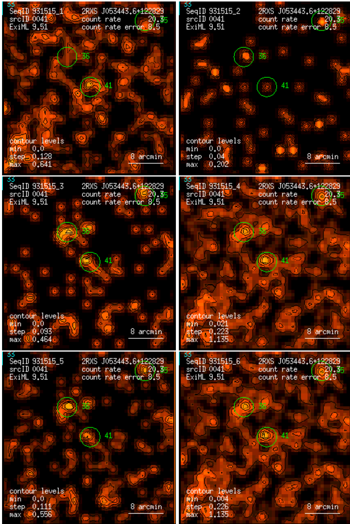
Figure 41: RASS 931515: detection 0041: band rate images, Gaussian filter: (1) PSPC channels 11 – 41, (2) 52 – 90, (3) 91 – 201, (4) 11 – 235, (5) 52 – 201, (6) 11 – 201. Broad band rates in counts/ks. Band rate contour levels in counts/ks/arcmin 2 .
