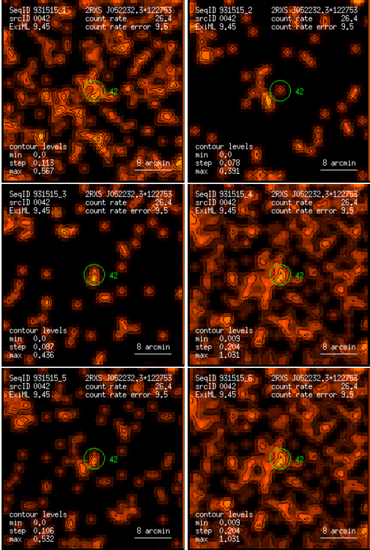
Figure 42: RASS 931515: detection 0042: band rate images, Gaussian filter: (1) PSPC channels 11 – 41, (2) 52 – 90, (3) 91 – 201, (4) 11 – 235, (5) 52 – 201, (6) 11 – 201. Broad band rates in counts/ks. Band rate contour levels in counts/ks/arcmin 2 .
