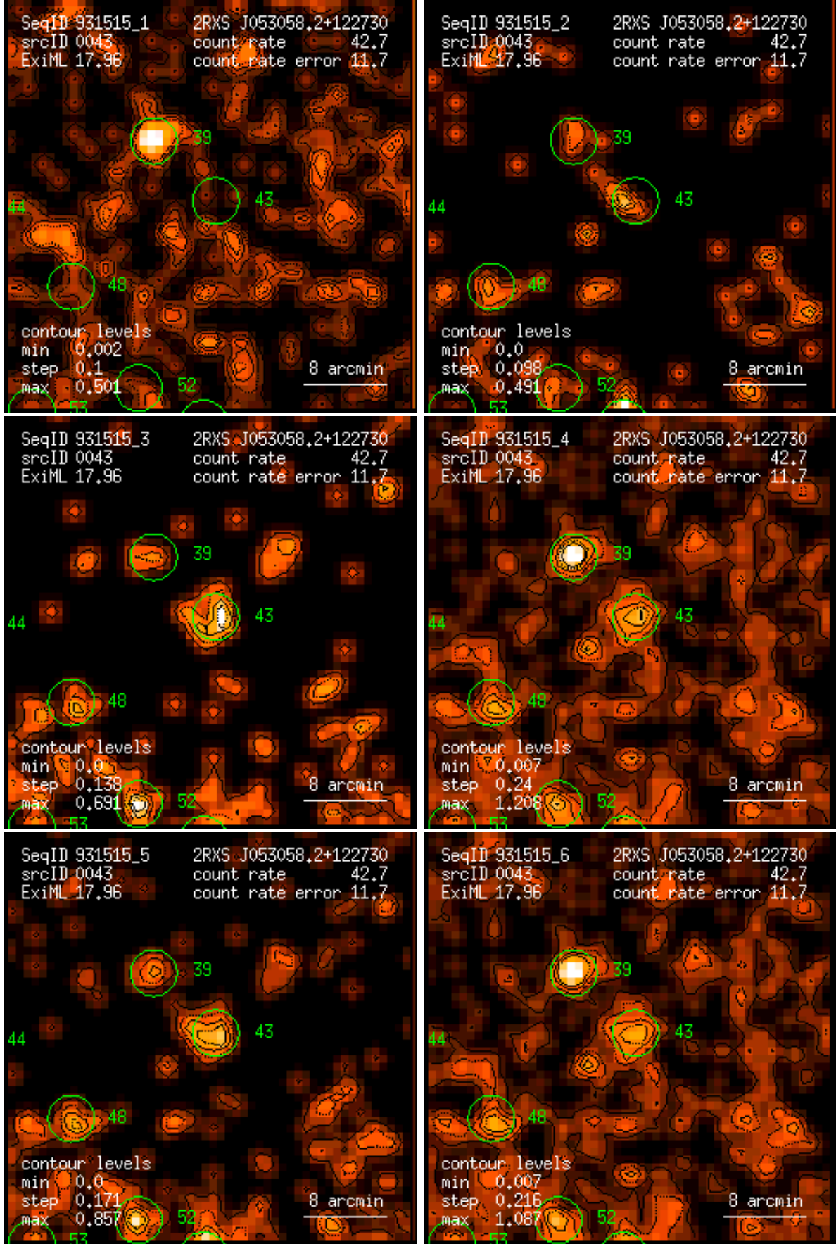
Figure 43: RASS 931515: detection 0043: band rate images, Gaussian filter: (1) PSPC channels 11 – 41, (2) 52 – 90, (3) 91 – 201, (4) 11 – 235, (5) 52 – 201, (6) 11 – 201. Broad band rates in counts/ks. Band rate contour levels in counts/ks/arcmin 2 .
