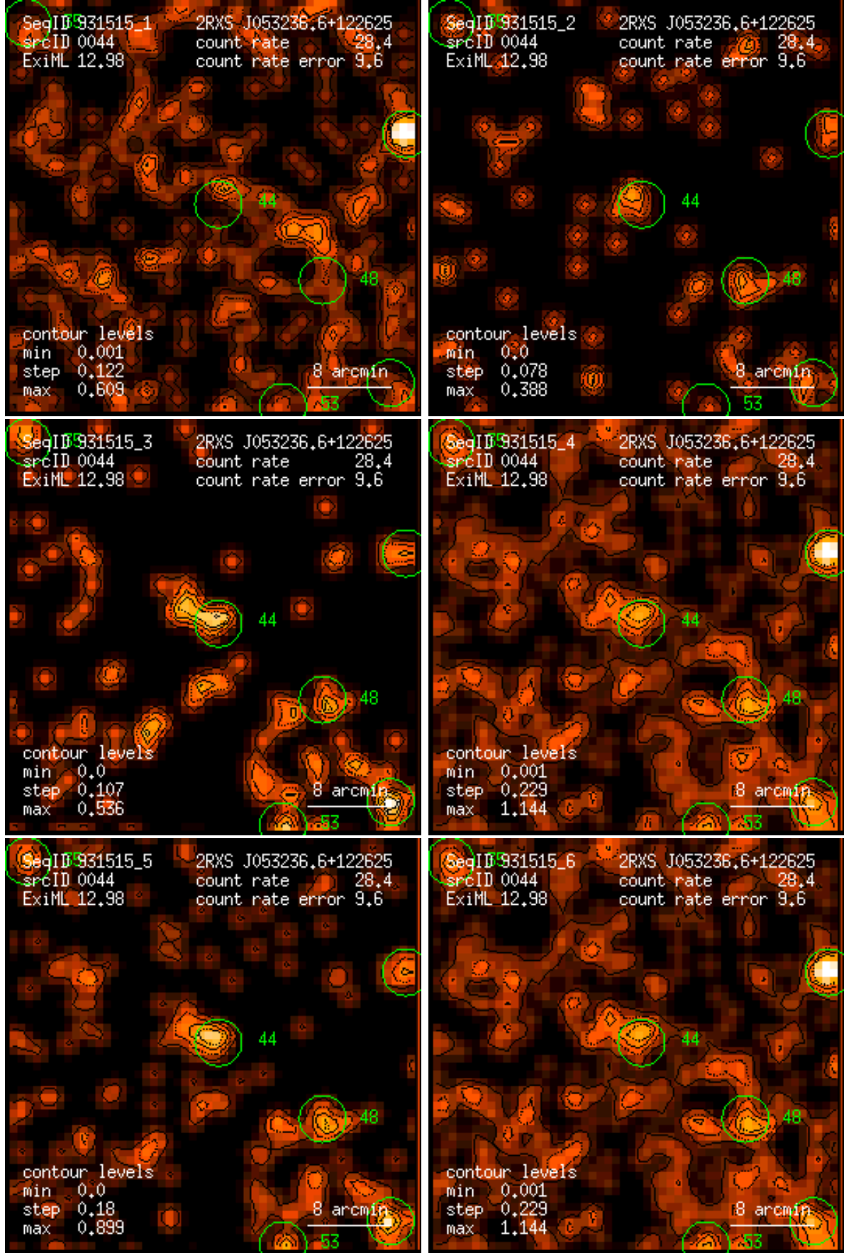
Figure 44: RASS 931515: detection 0044: band rate images, Gaussian filter: (1) PSPC channels 11 – 41, (2) 52 – 90, (3) 91 – 201, (4) 11 – 235, (5) 52 – 201, (6) 11 – 201. Broad band rates in counts/ks. Band rate contour levels in counts/ks/arcmin 2 .
