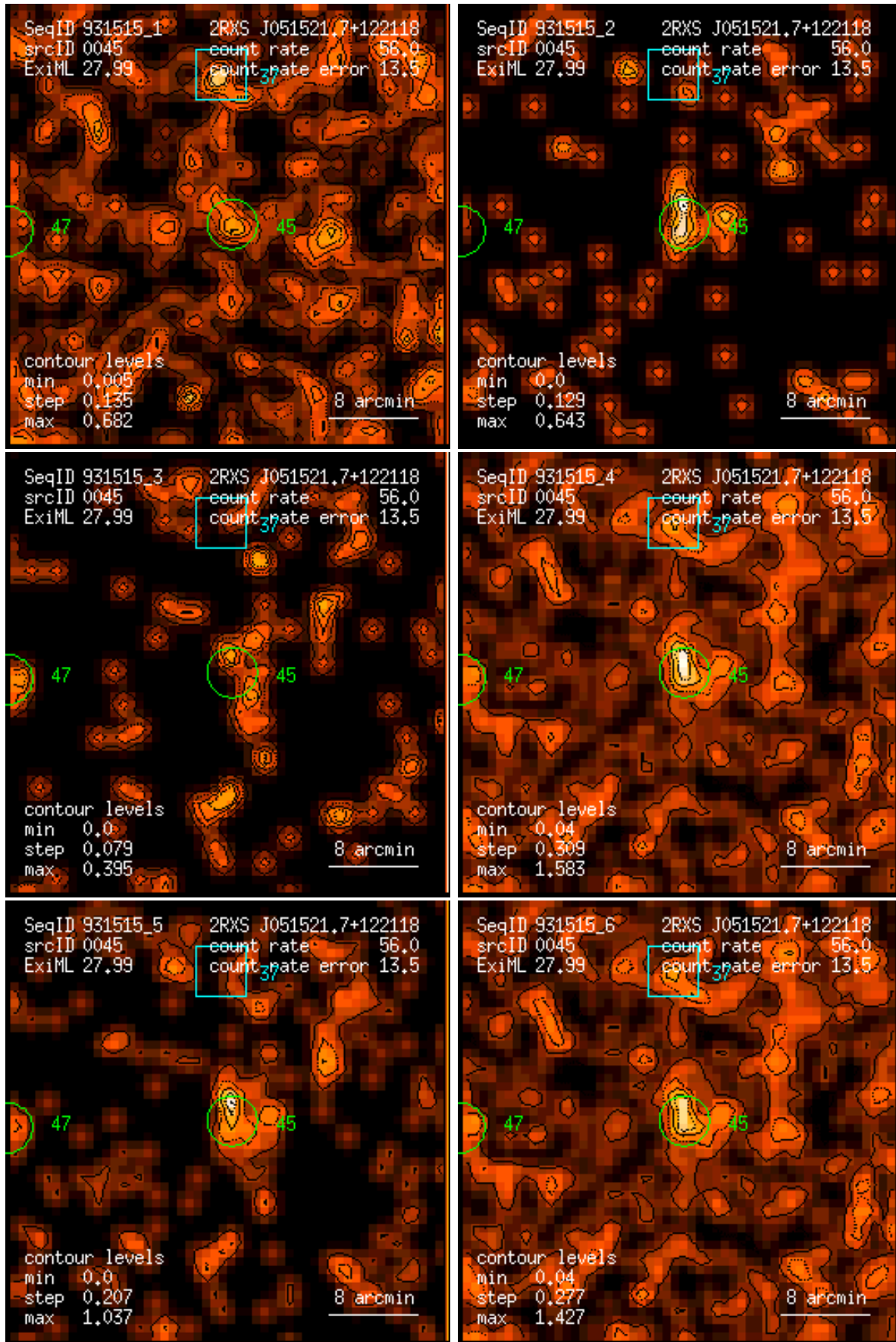
Figure 45: RASS 931515: detection 0045: band rate images, Gaussian filter: (1) PSPC channels 11 – 41, (2) 52 – 90, (3) 91 – 201, (4) 11 – 235, (5) 52 – 201, (6) 11 – 201. Broad band rates in counts/ks. Band rate contour levels in counts/ks/arcmin 2 .
