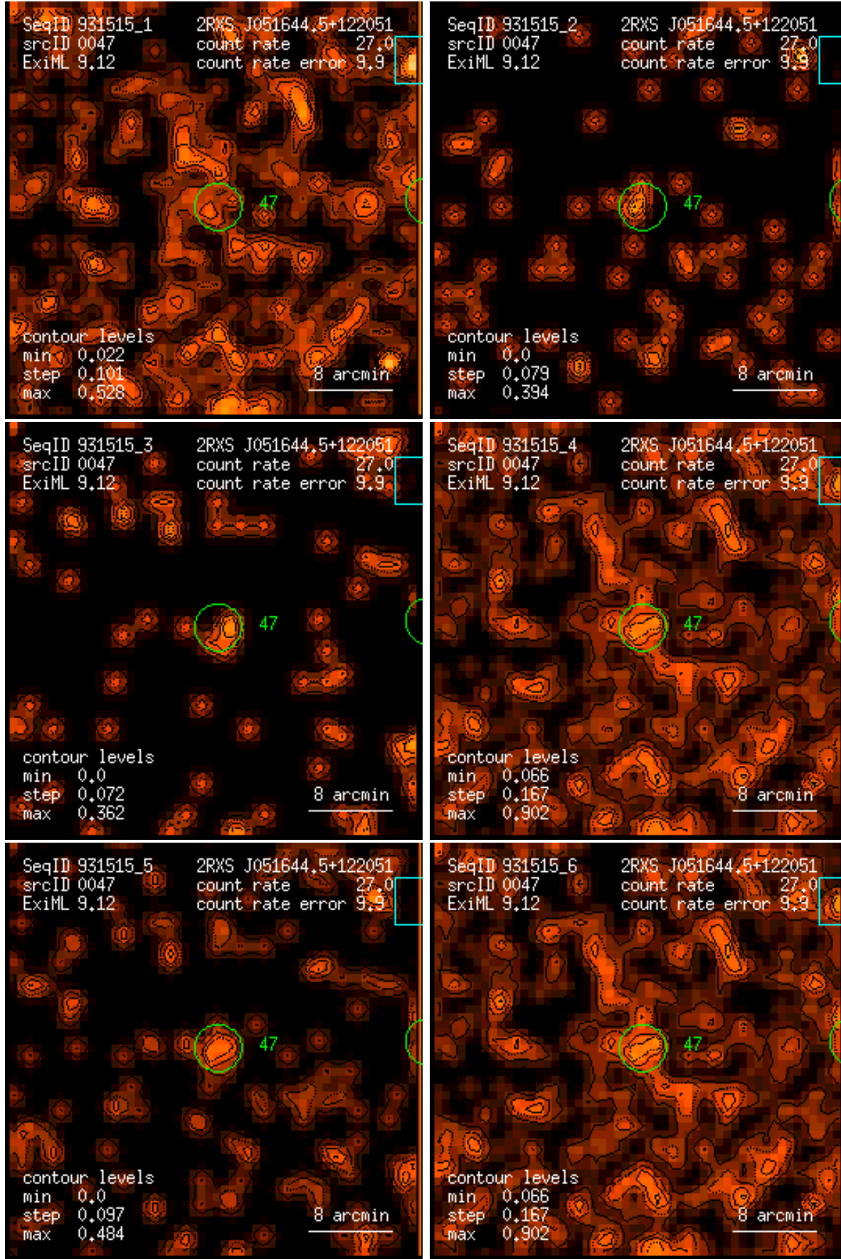
Figure 47: RASS 931515: detection 0047: band rate images, Gaussian filter: (1) PSPC channels 11 – 41, (2) 52 – 90, (3) 91 – 201, (4) 11 – 235, (5) 52 – 201, (6) 11 – 201. Broad band rates in counts/ks. Band rate contour levels in counts/ks/arcmin 2 .
