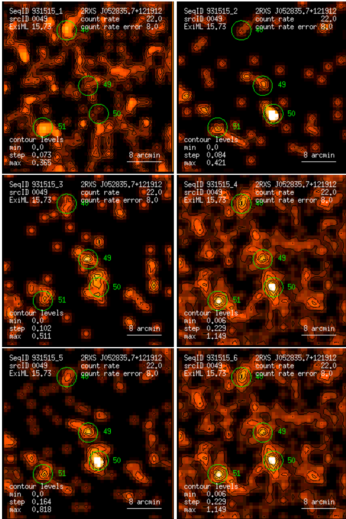
Figure 49: RASS 931515: detection 0049: band rate images, Gaussian filter: (1) PSPC channels 11 – 41, (2) 52 – 90, (3) 91 – 201, (4) 11 – 235, (5) 52 – 201, (6) 11 – 201. Broad band rates in counts/ks. Band rate contour levels in counts/ks/arcmin 2 .
