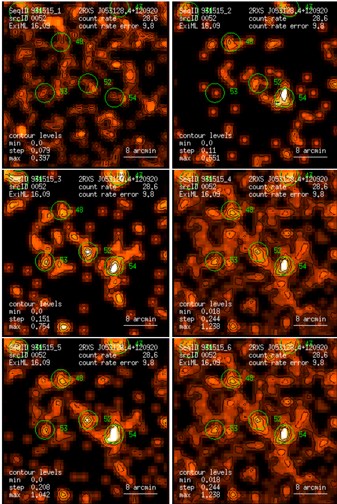
Figure 52: RASS 931515: detection 0052: band rate images, Gaussian filter: (1) PSPC channels 11 – 41, (2) 52 – 90, (3) 91 – 201, (4) 11 – 235, (5) 52 – 201, (6) 11 – 201. Broad band rates in counts/ks. Band rate contour levels in counts/ks/arcmin 2 .
