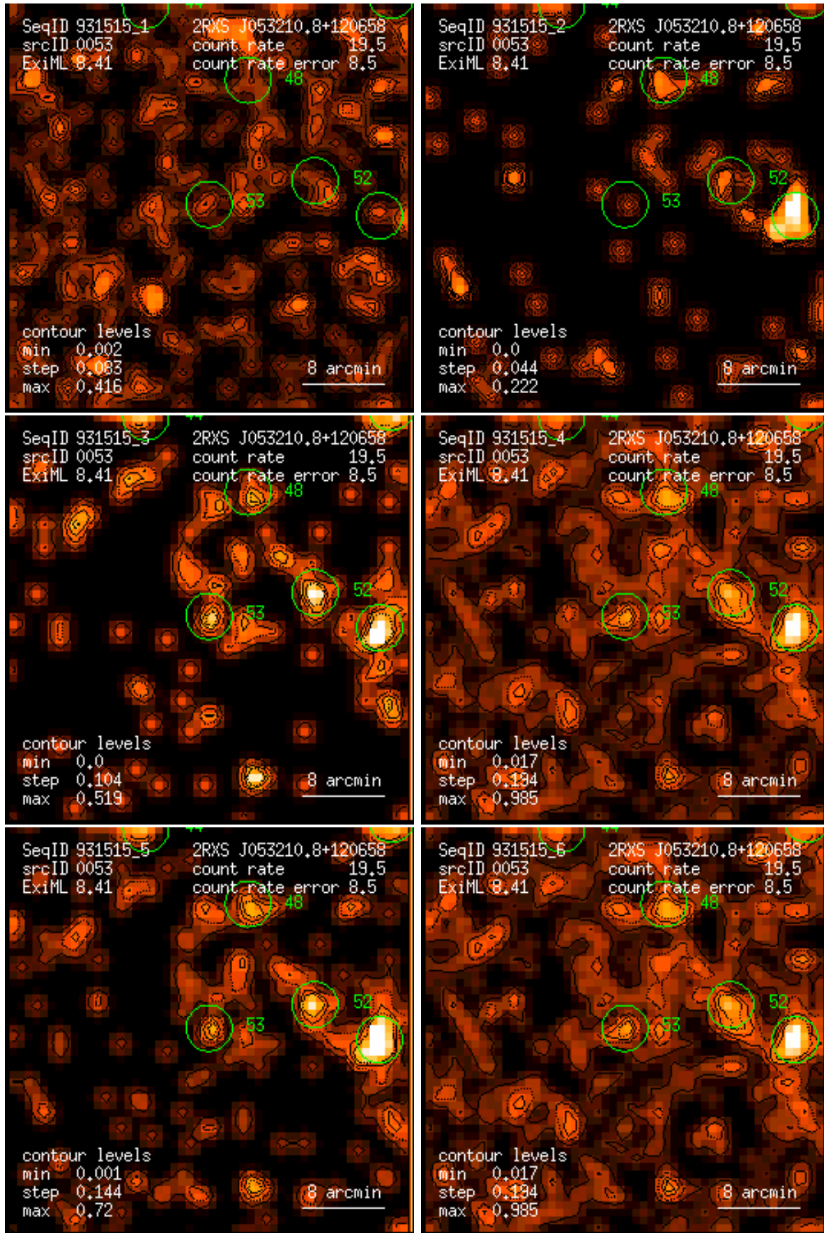
Figure 53: RASS 931515: detection 0053: band rate images, Gaussian filter: (1) PSPC channels 11 – 41, (2) 52 – 90, (3) 91 – 201, (4) 11 – 235, (5) 52 – 201, (6) 11 – 201. Broad band rates in counts/ks. Band rate contour levels in counts/ks/arcmin 2 .
