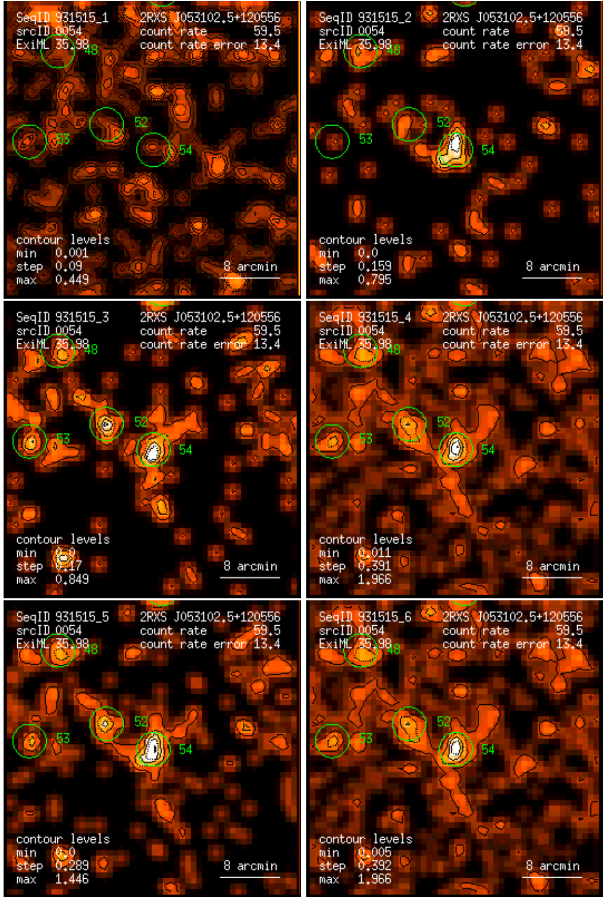
Figure 54: RASS 931515: detection 0054: band rate images, Gaussian filter: (1) PSPC channels 11 – 41, (2) 52 – 90, (3) 91 – 201, (4) 11 – 235, (5) 52 – 201, (6) 11 – 201. Broad band rates in counts/ks. Band rate contour levels in counts/ks/arcmin 2 .
