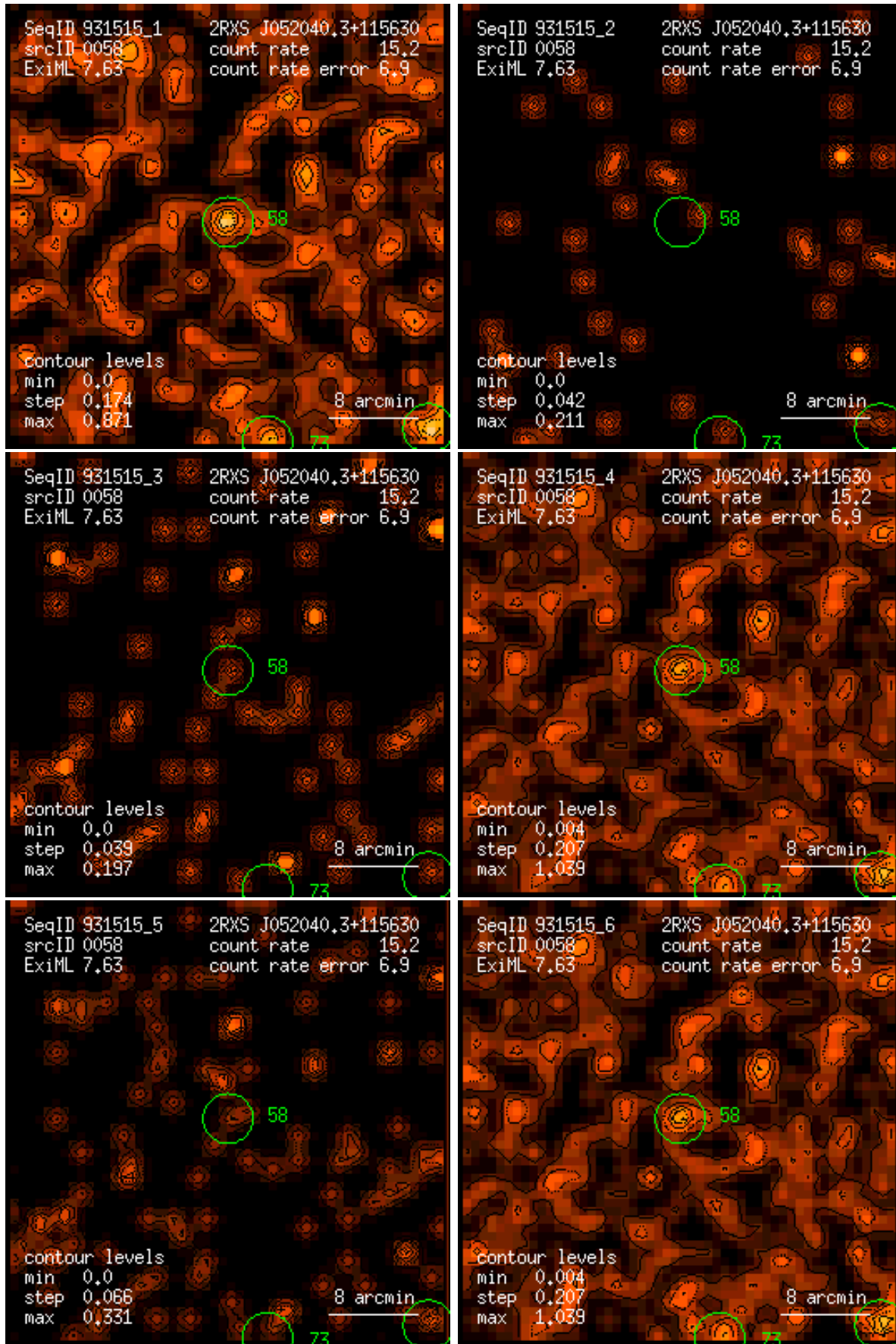
Figure 58: RASS 931515: detection 0058: band rate images, Gaussian filter: (1) PSPPC channels 11 – 41, (2) 52 – 90, (3) 91 – 201, (4) 11 – 235, (5) 52 – 201, (6) 11 – 201. Broad band rates in counts/ks. Band rate contour levels in counts/ks/arcmin 2 .
