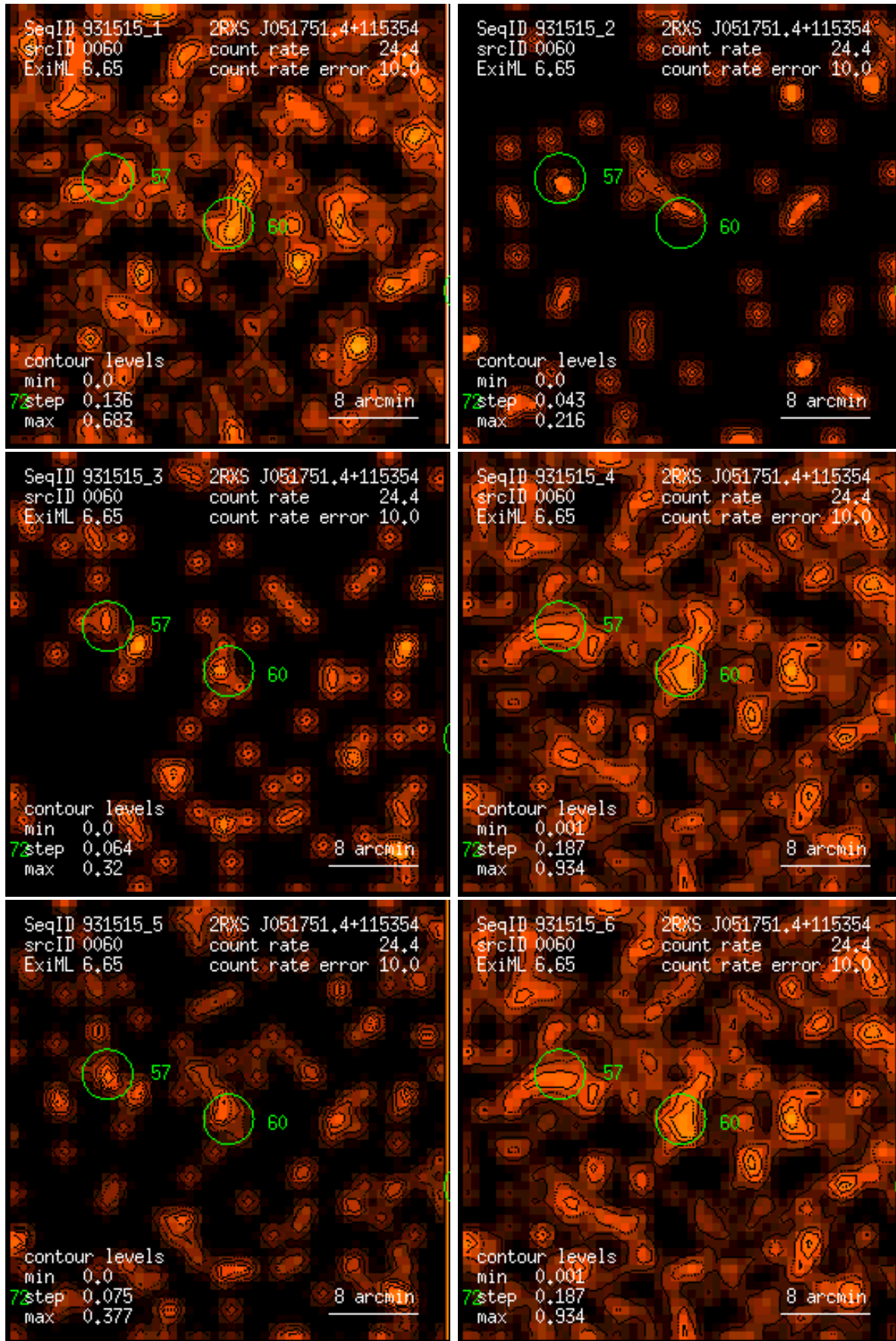
Figure 60: RASS 931515: detection 0060: band rate images, Gaussian filter: (1) PSPC channels 11 – 41, (2) 52 – 90, (3) 91 – 201, (4) 11 – 235, (5) 52 – 201, (6) 11 – 201. Broad band rates in counts/ks. Band rate contour levels in counts/ks/arcmin 2 .
