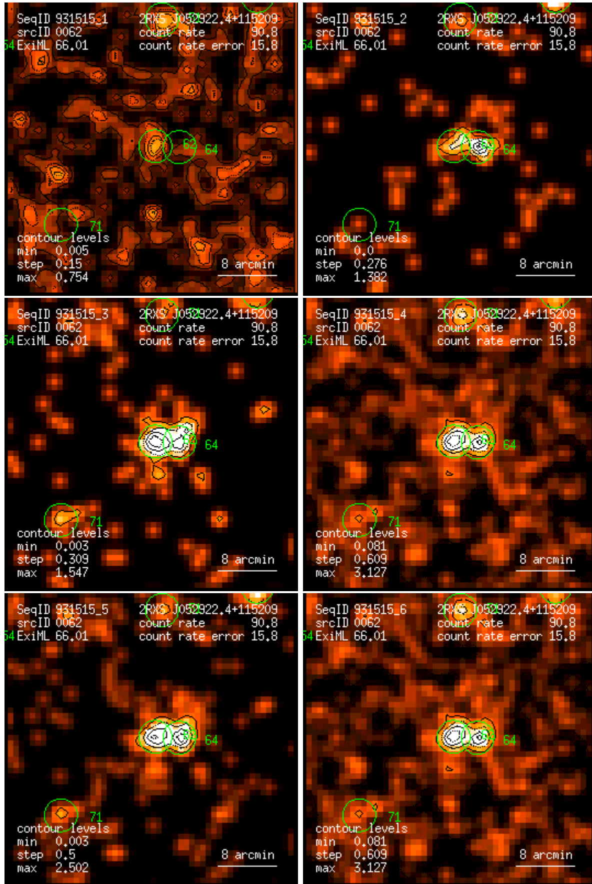
Figure 62: RASS 931515: detection 0062: band rate images, Gaussian filter: (1) PSPC channels 11 – 41, (2) 52 – 90, (3) 91 – 201, (4) 11 – 235, (5) 52 – 201, (6) 11 – 201. Broad band rates in counts/ks. Band rate contour levels in counts/ks/arcmin 2 .
