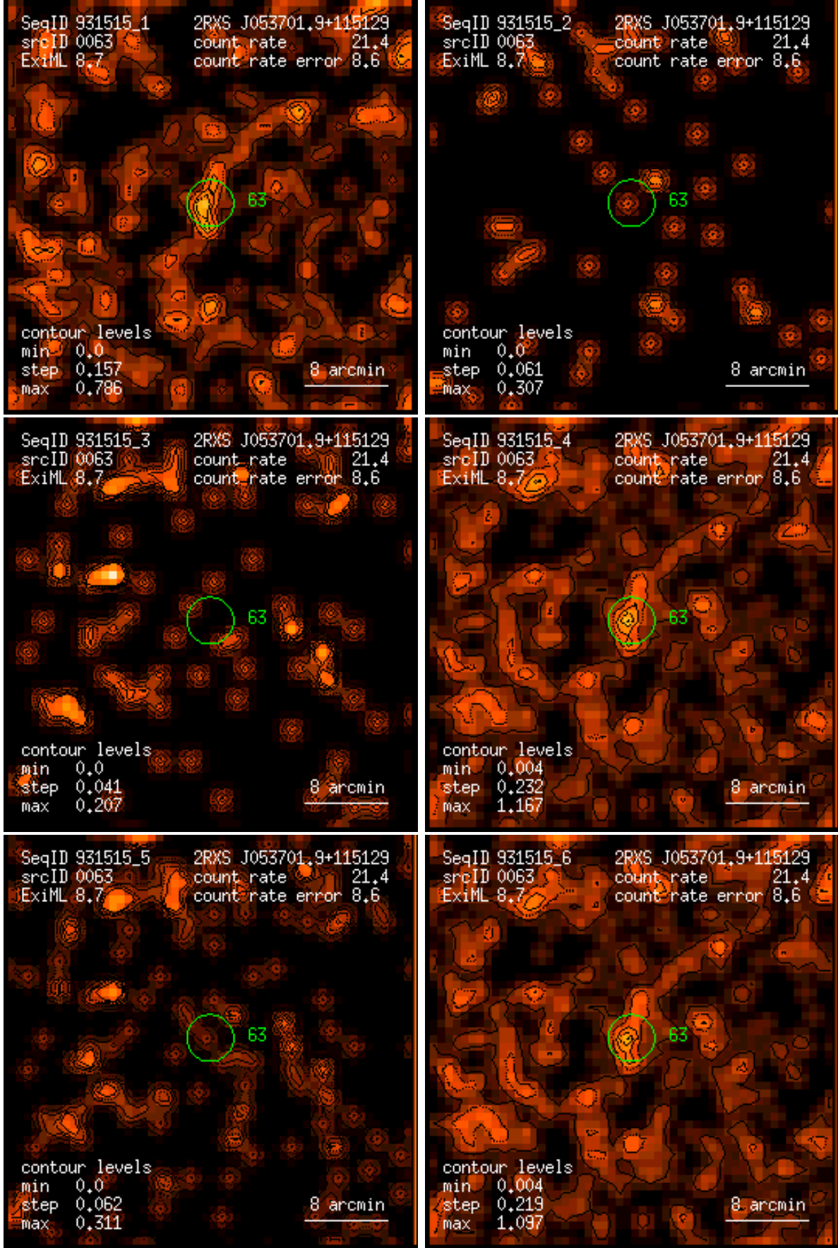
Figure 63: RASS 931515: detection 0063: band rate images, Gaussian filter: (1) PSPC channels 11 – 41, (2) 52 – 90, (3) 91 – 201, (4) 11 – 235, (5) 52 – 201, (6) 11 – 201. Broad band rates in counts/ks. Band rate contour levels in counts/ks/arcmin 2 .
