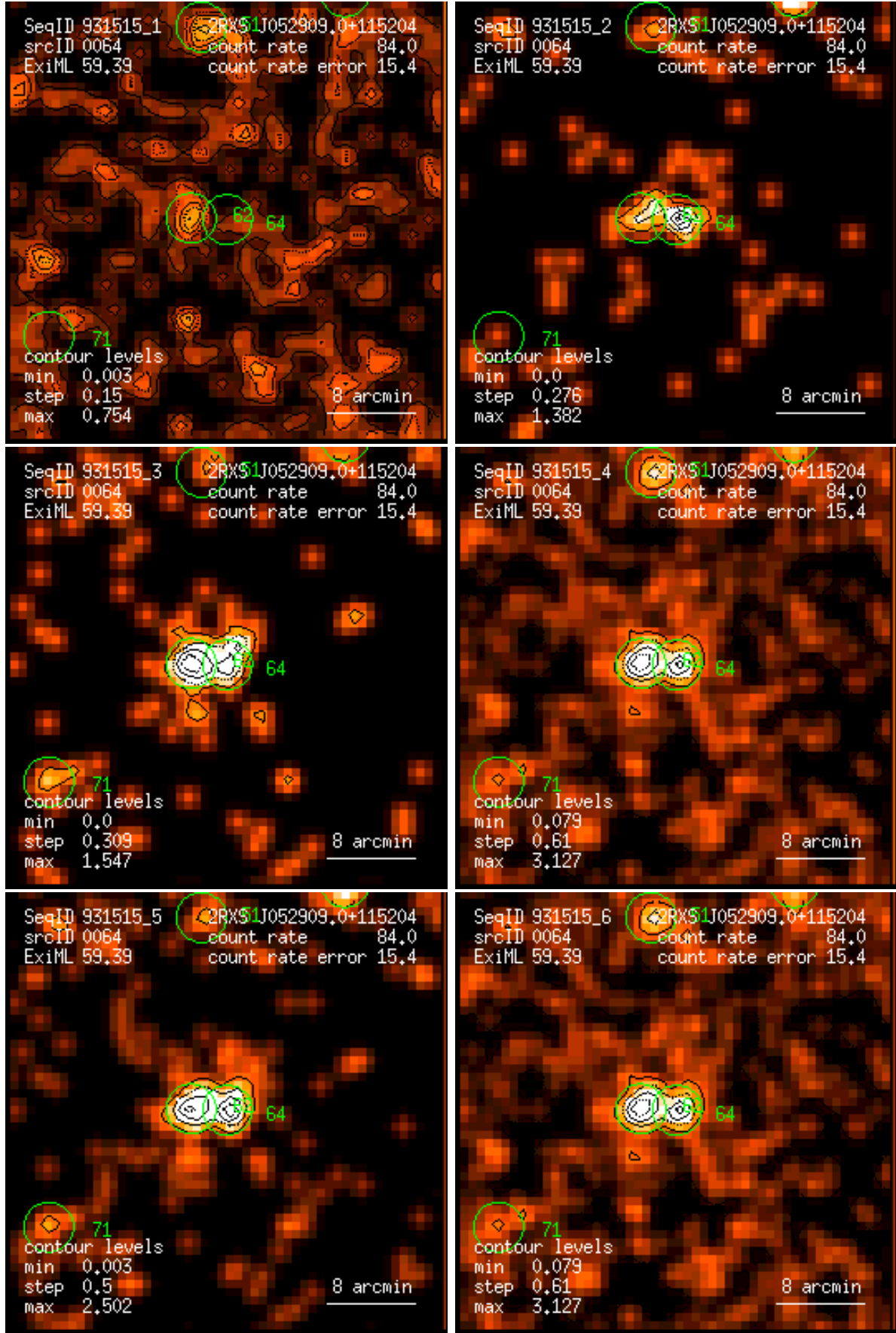
Figure 64: RASS 931515: detection 0064: band rate images, Gaussian filter: (1) PSPC channels 11 – 41, (2) 52 – 90, (3) 91 – 201, (4) 11 – 235, (5) 52 – 201, (6) 11 – 201. Broad band rates in counts/ks. Band rate contour levels in counts/ks/arcmin 2 .
