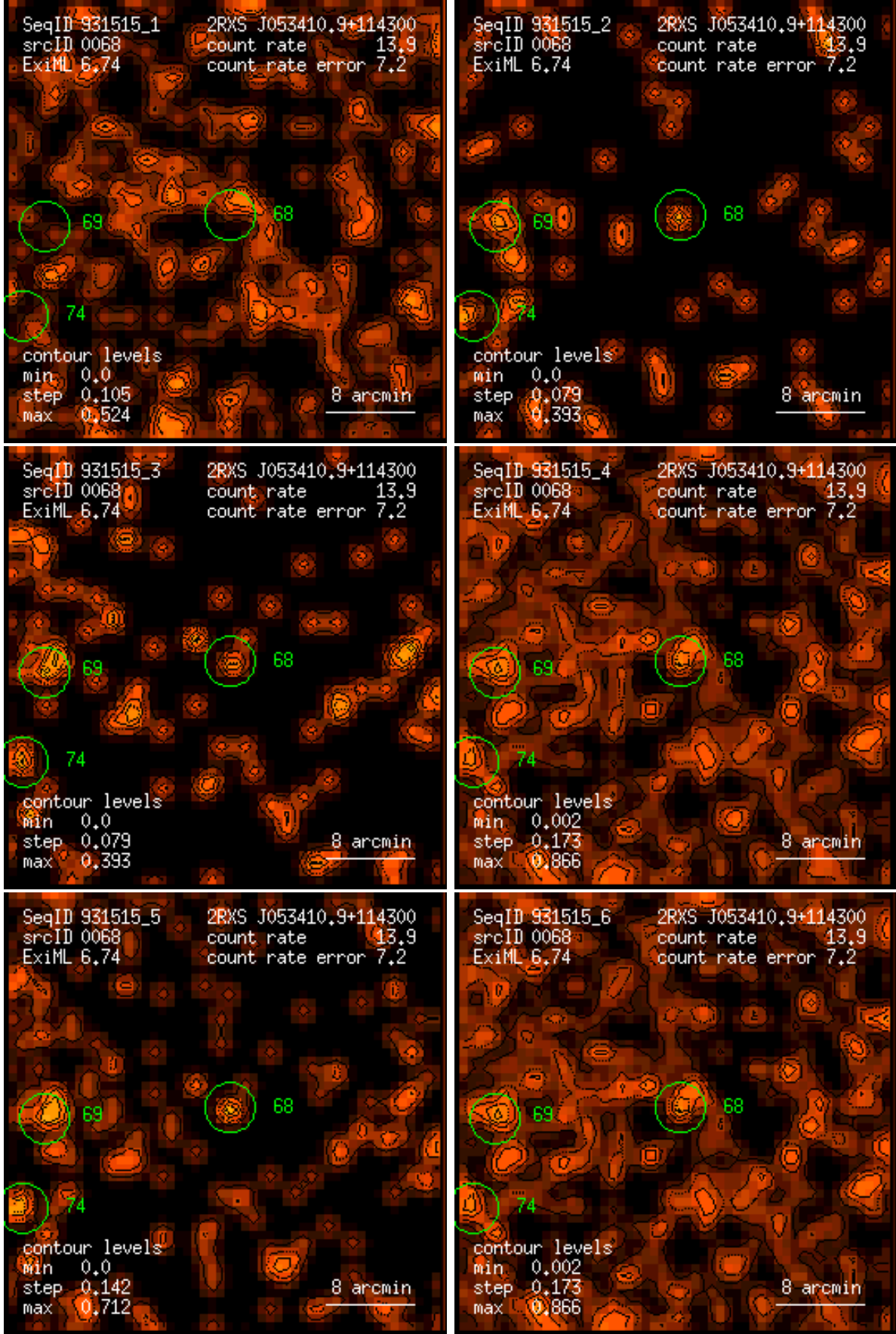
Figure 68: RASS 931515: detection 0068: band rate images, Gaussian filter: (1) PSPC channels 11 – 41, (2) 52 – 90, (3) 91 – 201, (4) 11 – 235, (5) 52 – 201, (6) 11 – 201. Broad band rates in counts/ks. Band rate contour levels in counts/ks/arcmin 2 .
