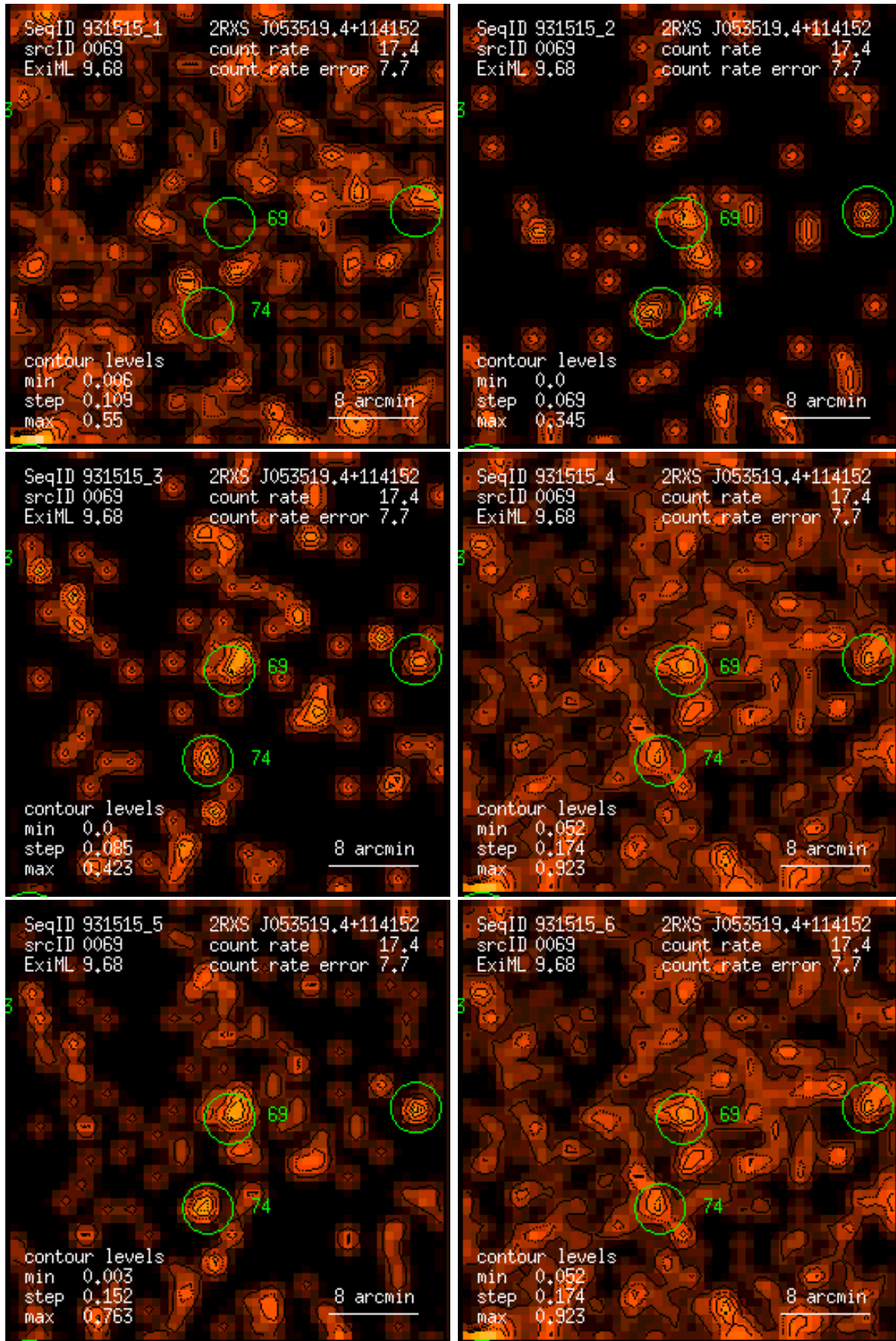
Figure 69: RASS 931515: detection 0069: band rate images, Gaussian filter: (1) PSPC channels 11 – 41, (2) 52 – 90, (3) 91 – 201, (4) 11 – 235, (5) 52 – 201, (6) 11 – 201. Broad band rates in counts/ks. Band rate contour levels in counts/ks/arcmin 2 .
