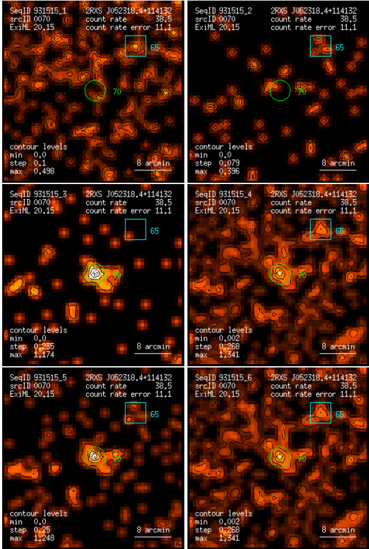
Figure 70: RASS 931515: detection 0070: band rate images, Gaussian filter: (1) PSPC channels 11 – 41, (2) 52 – 90, (3) 91 – 201, (4) 11 – 235, (5) 52 – 201, (6) 11 – 201. Broad band rates in counts/ks. Band rate contour levels in counts/ks/arcmin 2 .
