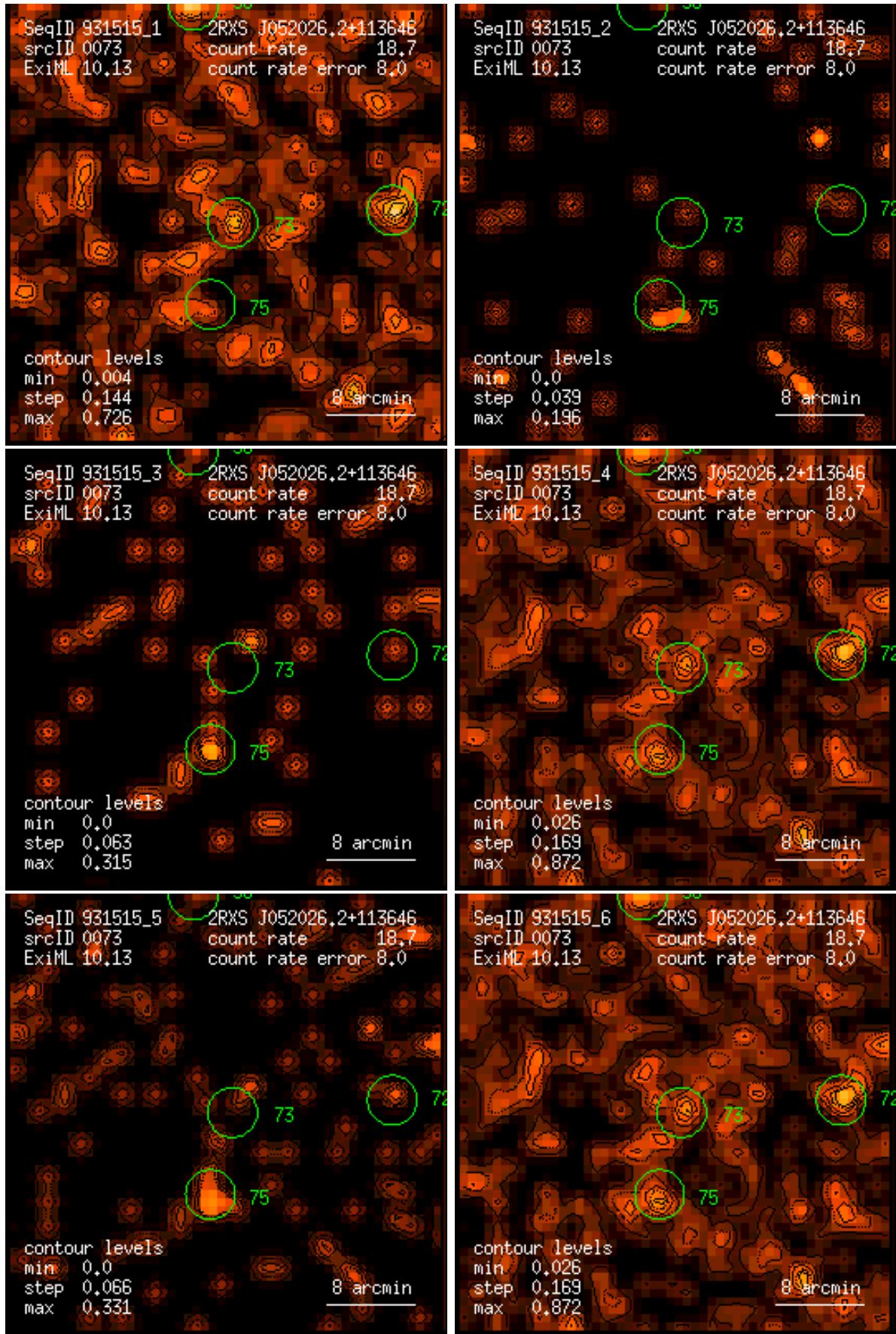
Figure 73: RASS 931515: detection 0073: band rate images, Gaussian filter: (1) PSPC channels 11 – 41, (2) 52 – 90, (3) 91 – 201, (4) 11 – 235, (5) 52 – 201, (6) 11 – 201. Broad band rates in counts/ks. Band rate contour levels in counts/ks/arcmin 2 .
