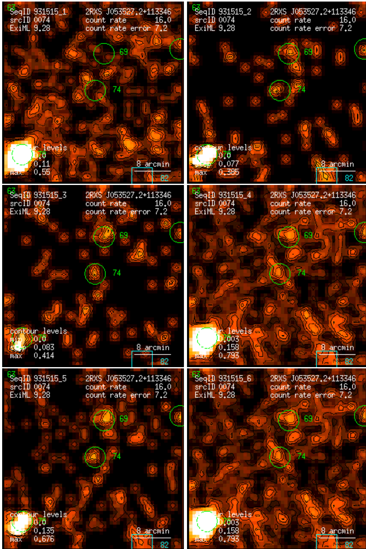
Figure 74: RASS 931515: detection 0074: band rate images, Gaussian filter: (1) PSPC channels 11 – 41, (2) 52 – 90, (3) 91 – 201, (4) 11 – 235, (5) 52 – 201, (6) 11 – 201. Broad band rates in counts/ks. Band rate contour levels in counts/ks/arcmin 2 .
