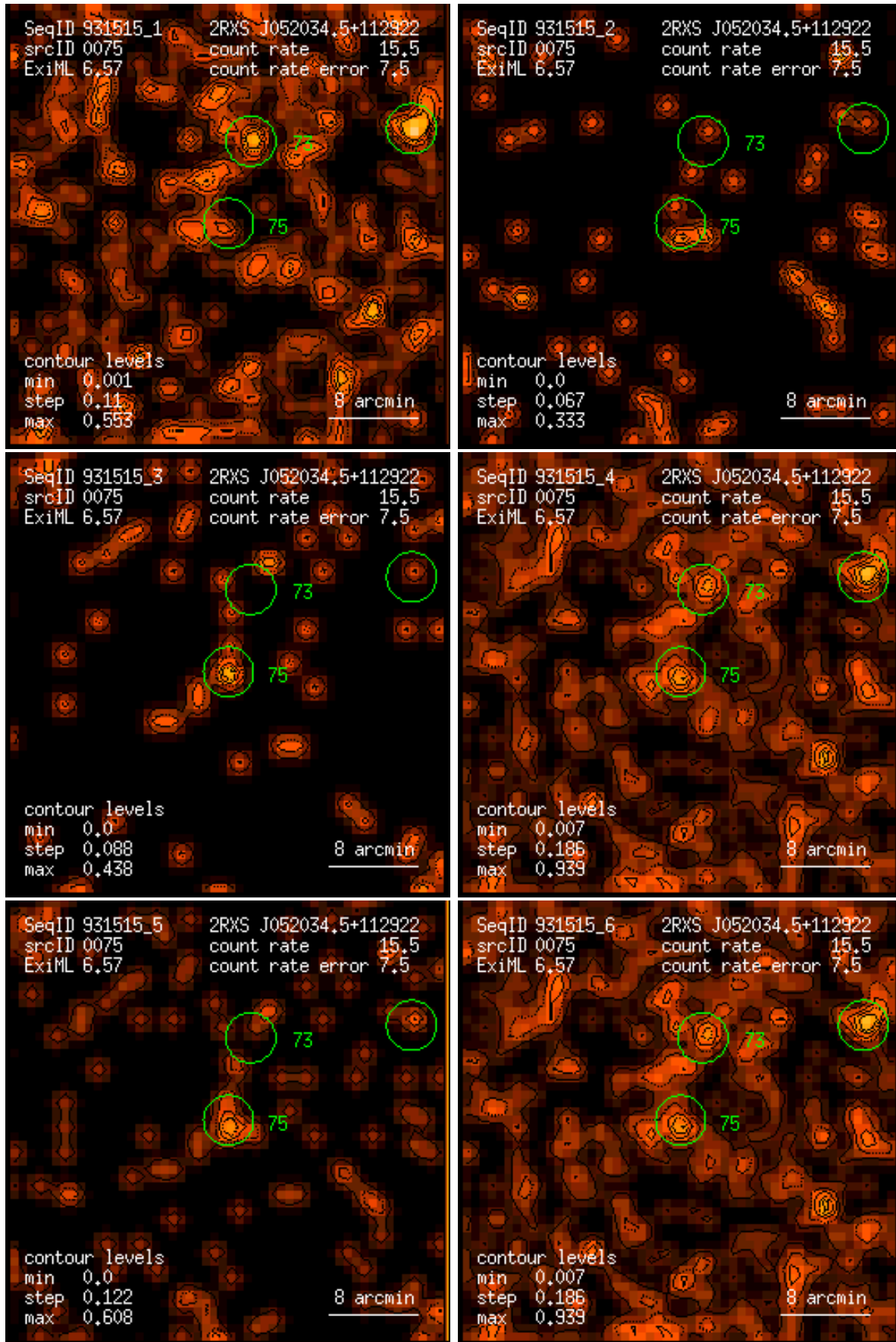
Figure 75: RASS 931515: detection 0075: band rate images, Gaussian filter: (1) PSPC channels 11 – 41, (2) 52 – 90, (3) 91 – 201, (4) 11 – 235, (5) 52 – 201, (6) 11 – 201. Broad band rates in counts/ks. Band rate contour levels in counts/ks/arcmin 2 .
