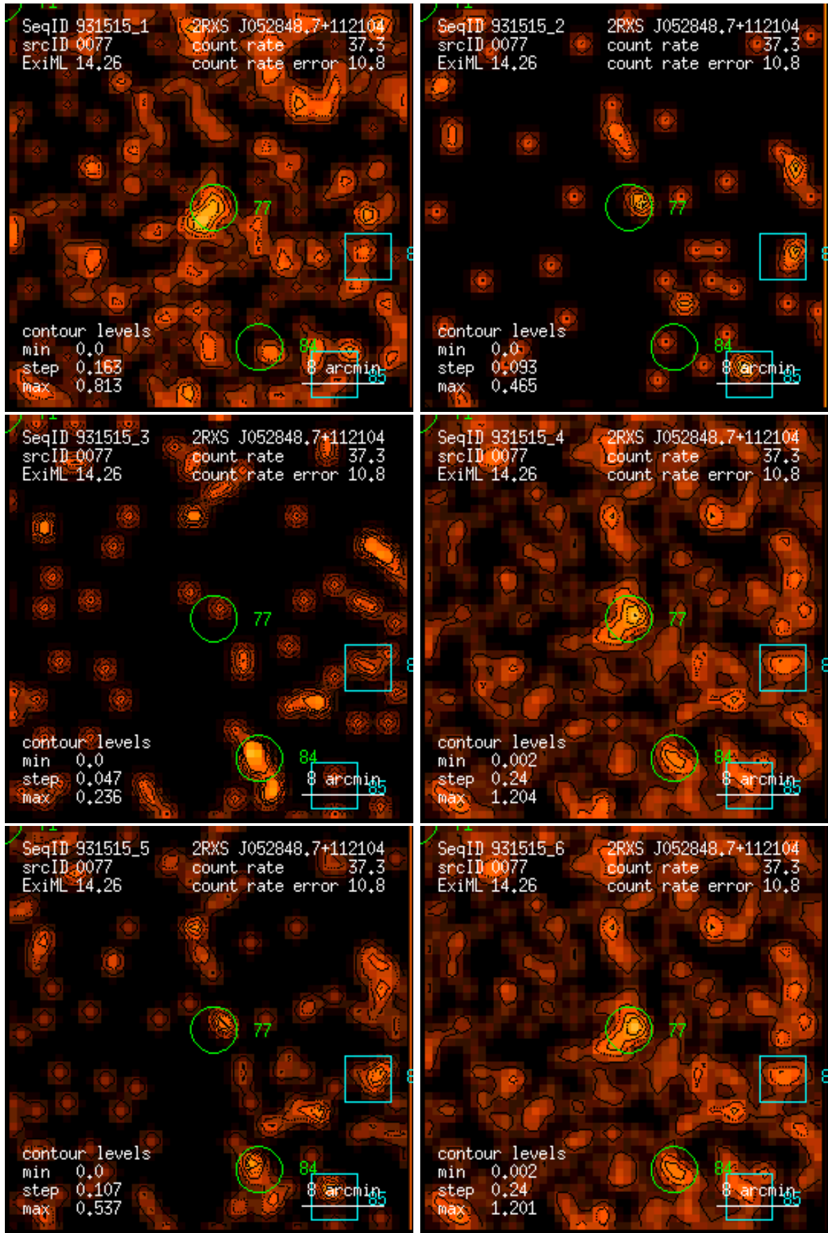
Figure 77: RASS 931515: detection 0077: band rate images, Gaussian filter: (1) PSPC channels 11 – 41, (2) 52 – 90, (3) 91 – 201, (4) 11 – 235, (5) 52 – 201, (6) 11 – 201. Broad band rates in counts/ks. Band rate contour levels in counts/ks/arcmin 2 .
