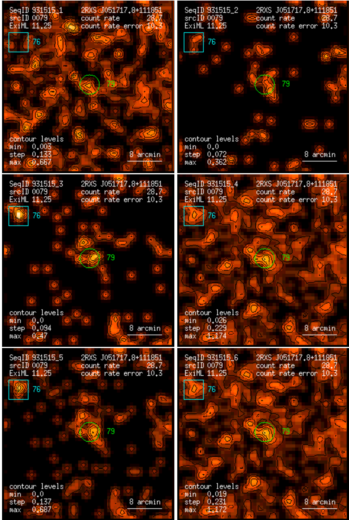
Figure 79: RASS 931515: detection 0079: band rate images, Gaussian filter: (1) PSPC channels 11 – 41, (2) 52 – 90, (3) 91 – 201, (4) 11 – 235, (5) 52 – 201, (6) 11 – 201. Broad band rates in counts/ks. Band rate contour levels in counts/ks/arcmin 2 .
